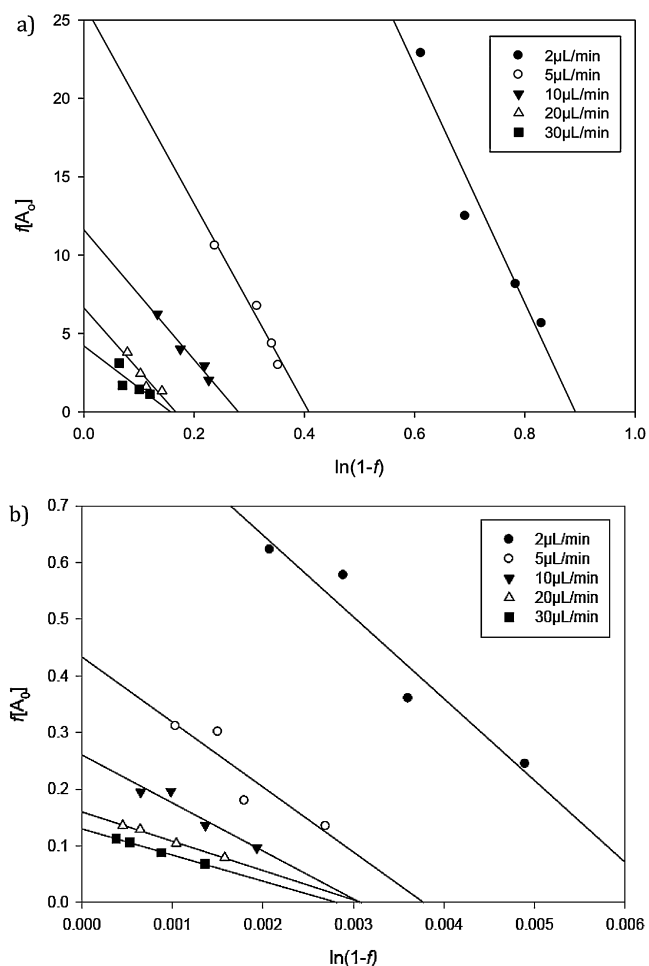
Fig. 7. Kinetics determination using Lilly–Hornby model for continuous-flow mode reaction. Data to obtain these plots was taken from Fig. 6. (a) TK-catalyzed reaction and (b) TAM-catalyzed reaction. Solid lines fitted by linear regression. Values of K_{m(\text{app})} and C for the continuous flow reactions could be obtained from these plots.
