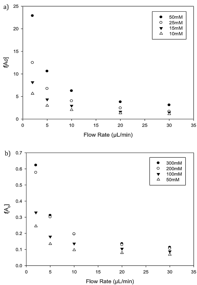
Fig. 6. Bioconversions using different substrate concentration at flow rates ranging from 2 \mu\text{L}/\text{min} to 30 \mu\text{L}/\text{min} . (a) Continuous-flow TK-catalyzed reaction at different GA concentration (10–50 mM) with HPA concentration was kept at 100 mM. (b) Continuous-flow TAM-catalyzed reaction at different ERY concentration (50–300 mM) with MBA concentration was kept at 10 mM. Concentration of immobilized TK and TAM was \sim 0.05 mg/mL and 0.4 mg/mL respectively.
