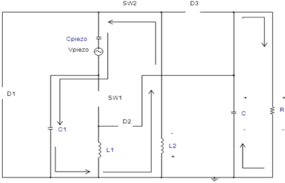
Figure-5. Mode 3 operation of voltage doubler.
