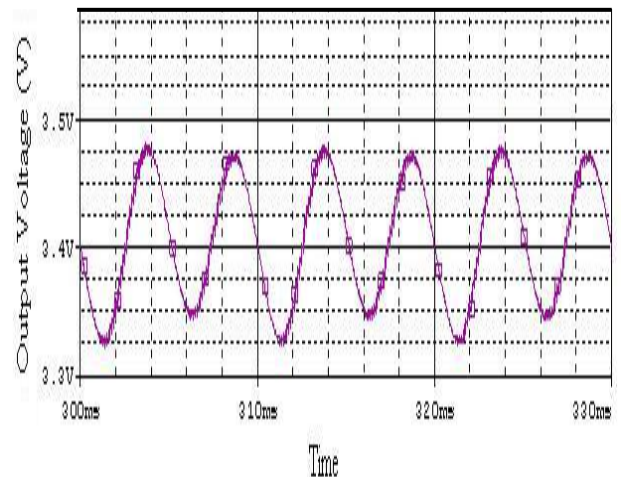
Figure-7. Output voltage vs time.
