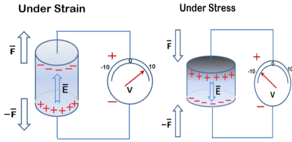
Figure-1. Basic principle of piezo-energy generation.
