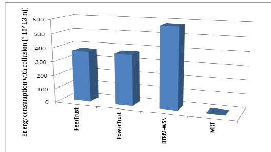
Figure 10: Comparison between MRT model and existing trust and reputation models in terms of energy consumption with collusion
