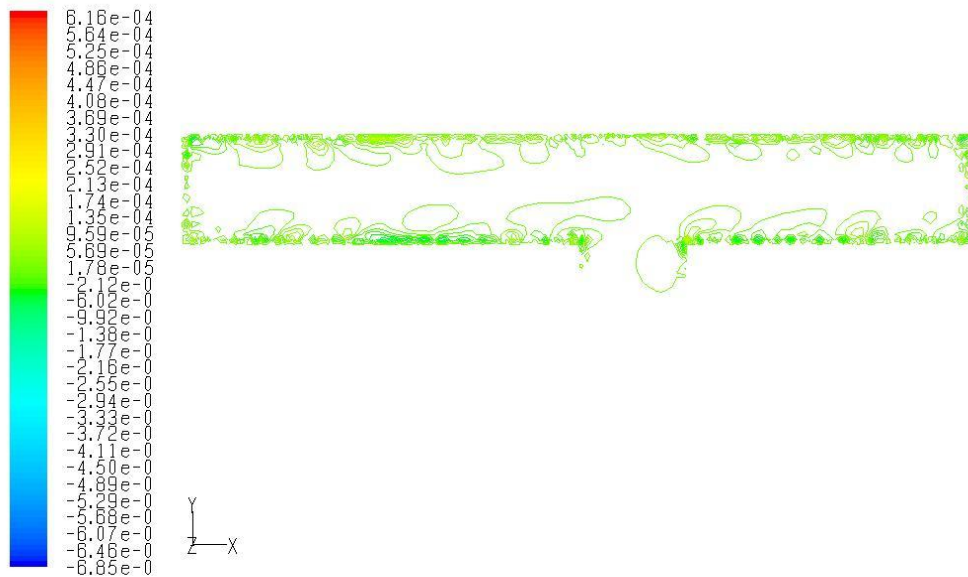
Contours of Z Velocity (m/s) Apr 09, 2008 FLUENT 6.3 (3d, dp, pbns, lam)
