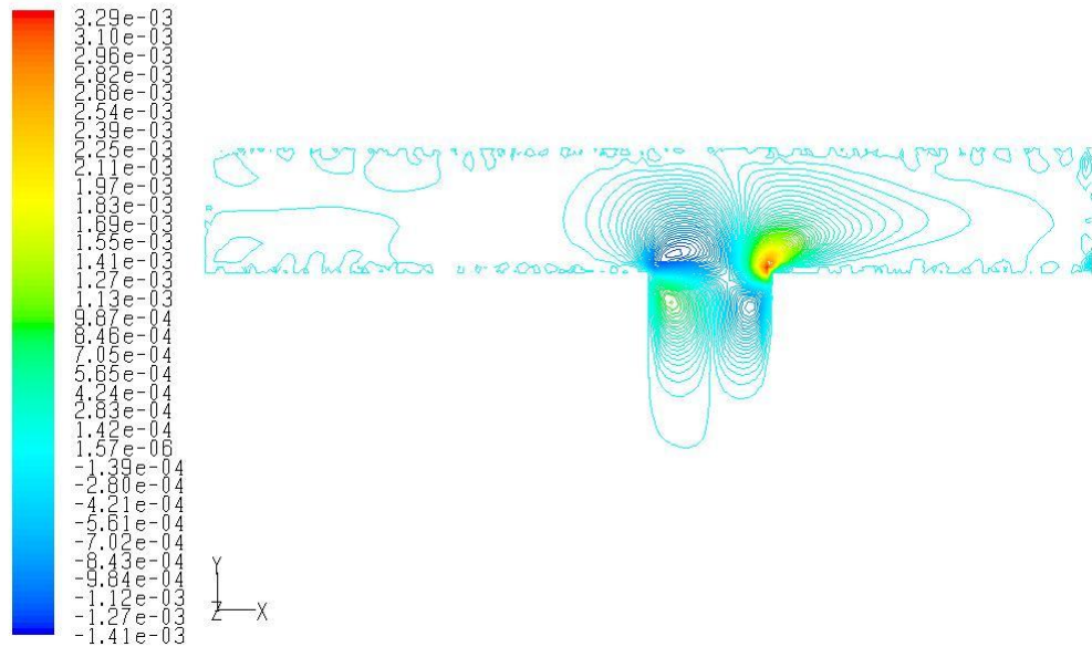
Contours of Y Velocity (m/s) Apr 09, 2008 FLUENT 6.3 (3d, dp, pbns, lam)
