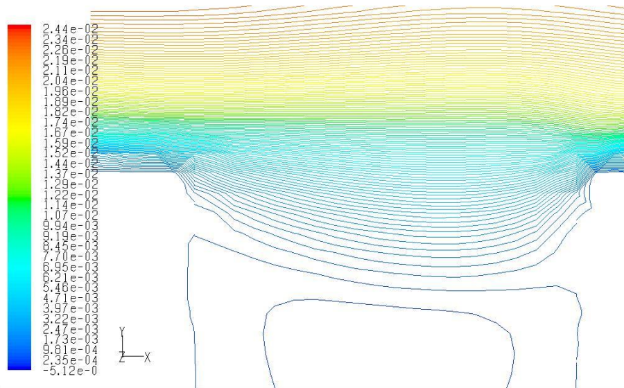
Contours of X Velocity (m/s)
