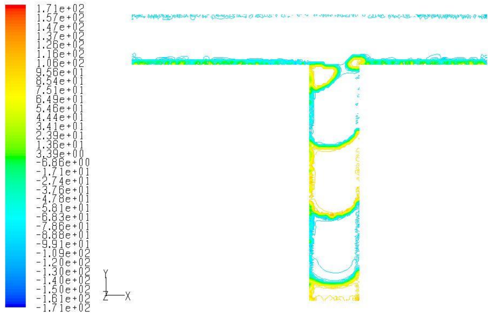
Contours of Velocity Angle (deg) Apr 09, 2008 FLUENT 6.3 (3d, dp, pbns, lam)
