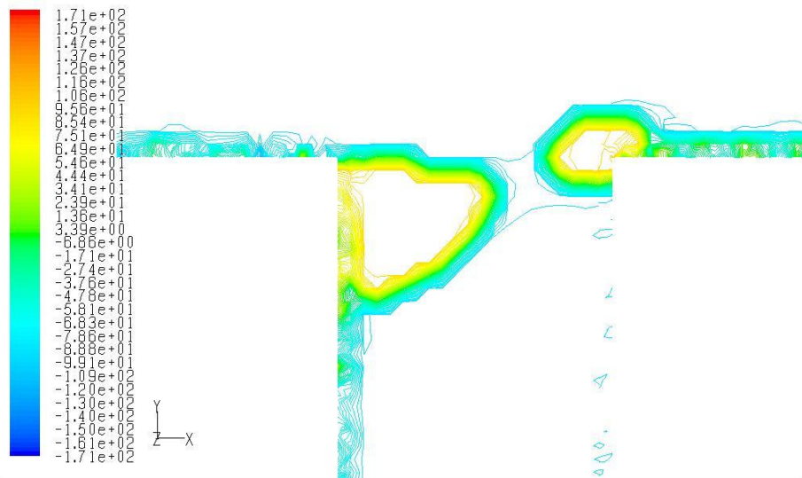
Contours of Velocity Angle (deg) Apr 09, 2008 FLUENT 6.3 (3d, dp, pbns, lam)
