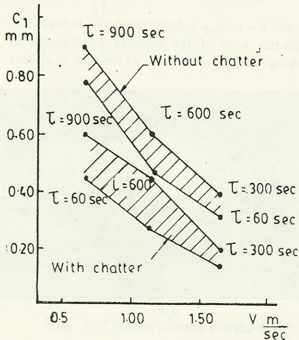
Fig. 8 Dependence of chip-tool plastic contact length C_1 and total length, C on cutting speed V at different intensities of chatter.
