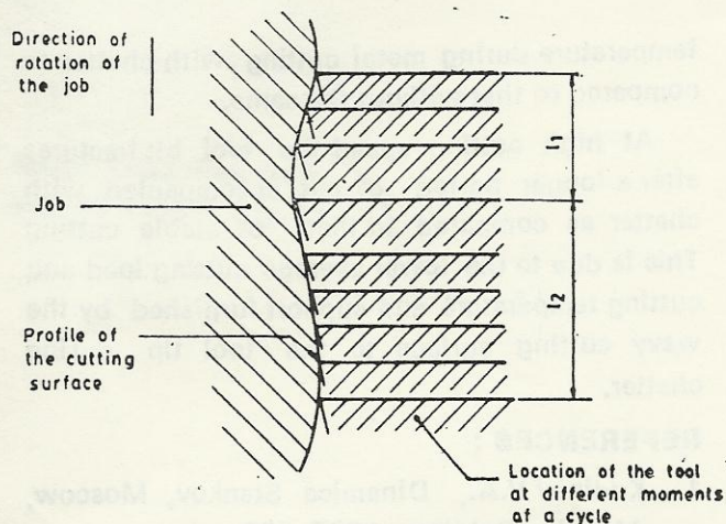
Fig. 10 Relative location of the tool and wavy cutting surface at various moments of cut during intensive chatter. Cutting speed, V=1.67 m/sec
