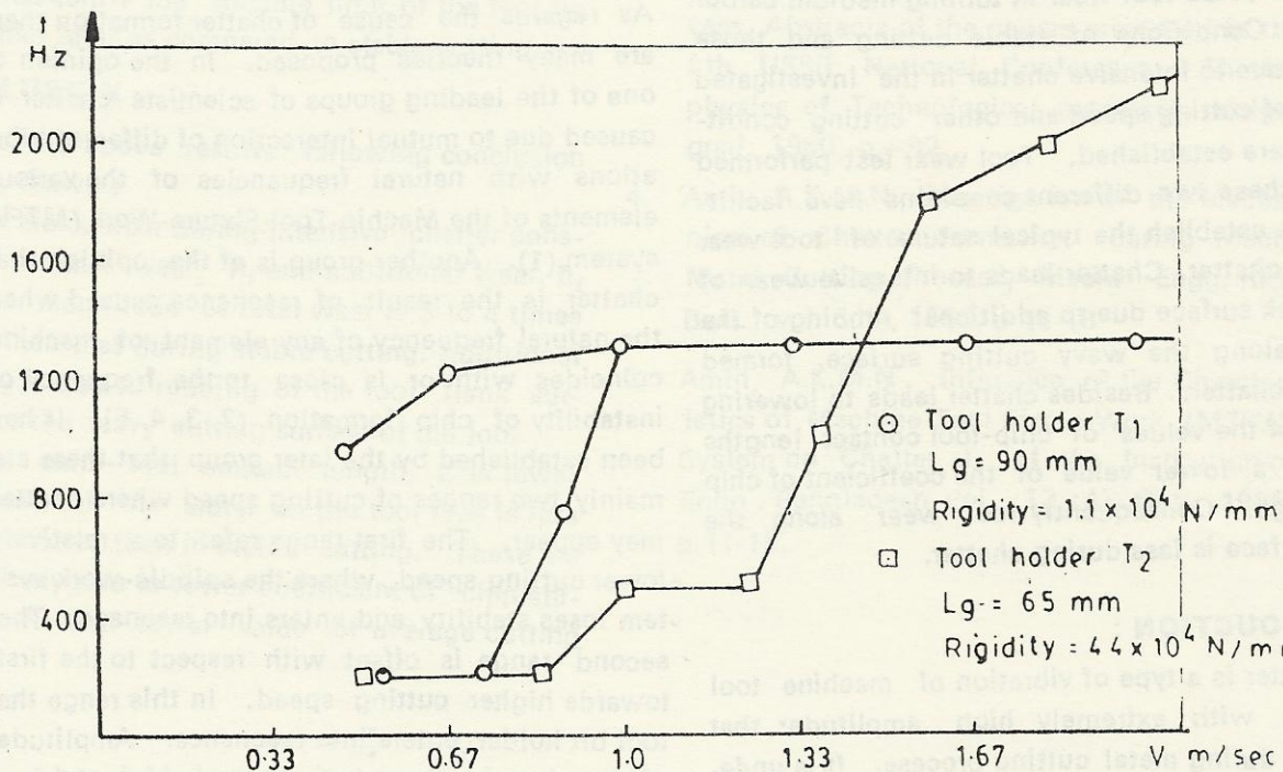
Fig. 1. Influence of tool bit holder on the orientation of the second horizontal portion of the chatter frequency versus cutting speed curve, f=\varphi(V) .
