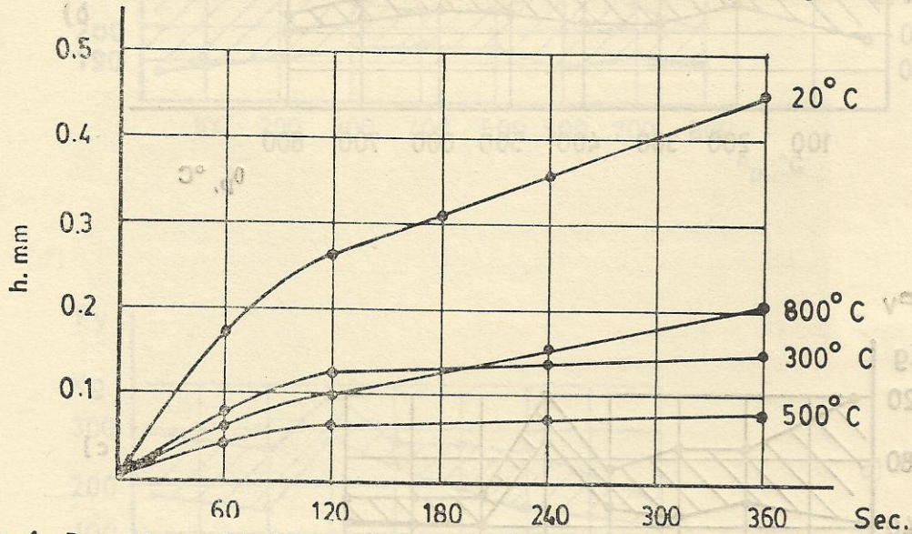
Fig. 4. Dependence of tool wear, h on preheating temperature in machining BT 3-1.
