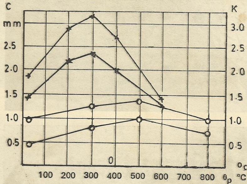
(d) Fig. 10. Dependence of chip-tool contact length, C and coefficient of chip shrinkage K on preheating temperature, \theta_p .
