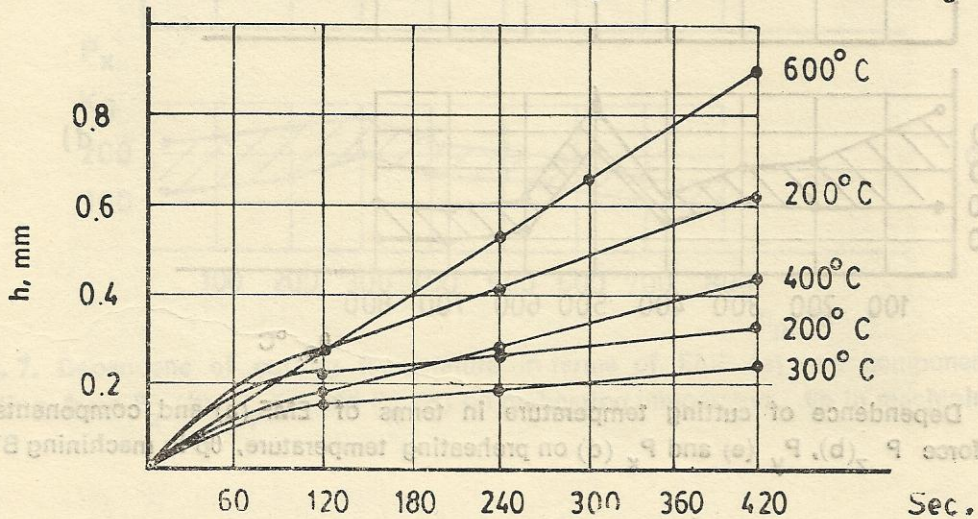
Fig. 5. Dependence of tool wear, h on preheating temperature in machining 3N-481
