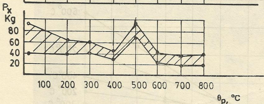
Fig. 6. Dependence of cutting temperature in terms of EMF (a) and components of cutting force P_z (b), P_y (e) and P_x (d) on preheating temperature, \theta_p in machining BT-3-1.
