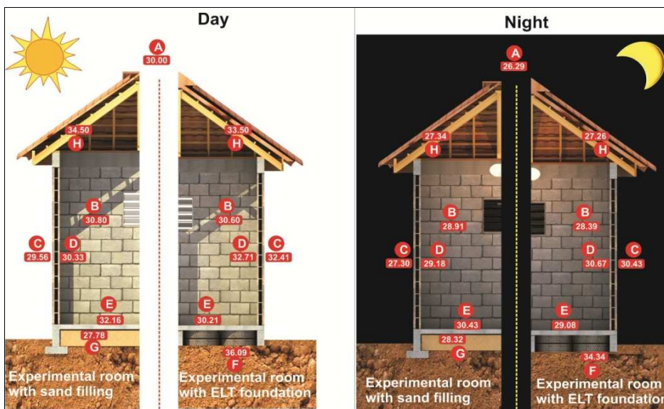
Figure 3: Indoor and Outdoor temperature variations (February 2012)
