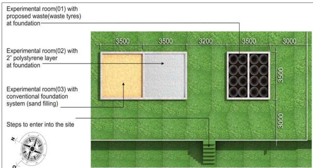
Figure 2: Plan of experimental set-up
