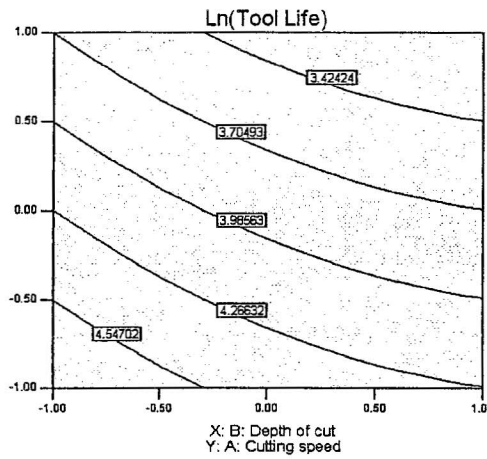
Figure 2: Contour plot on 3-D contour RSM response surface plot with the maximum and minimum values of tool life (TL) [Design point: TL=4.83@125min, V=-1.00@40\text{m/min} , d=-1.00@0.6\text{m/min} , f=0.83@0.027\text{mm/tooth} ]
