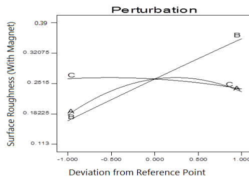
Fig. 3: Perturbation plot for surface roughness
