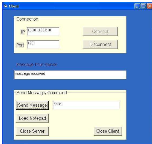
Figure 7. Chatting from client side (LPMS).
