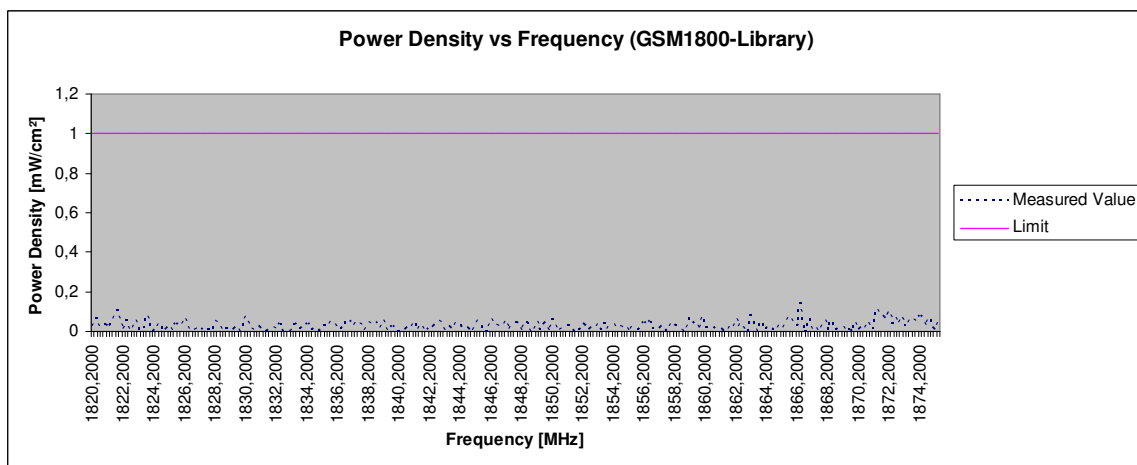
Fig. 3: Power density measured at central library for GSM1800 signals
