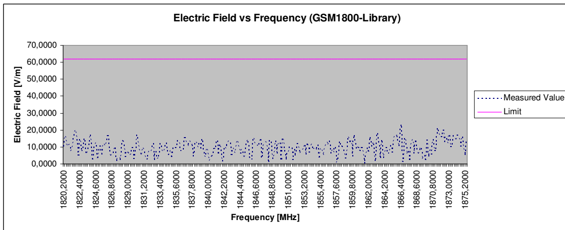
Fig. 2: Electric field intensity measured at central library for GSM1800 signals
