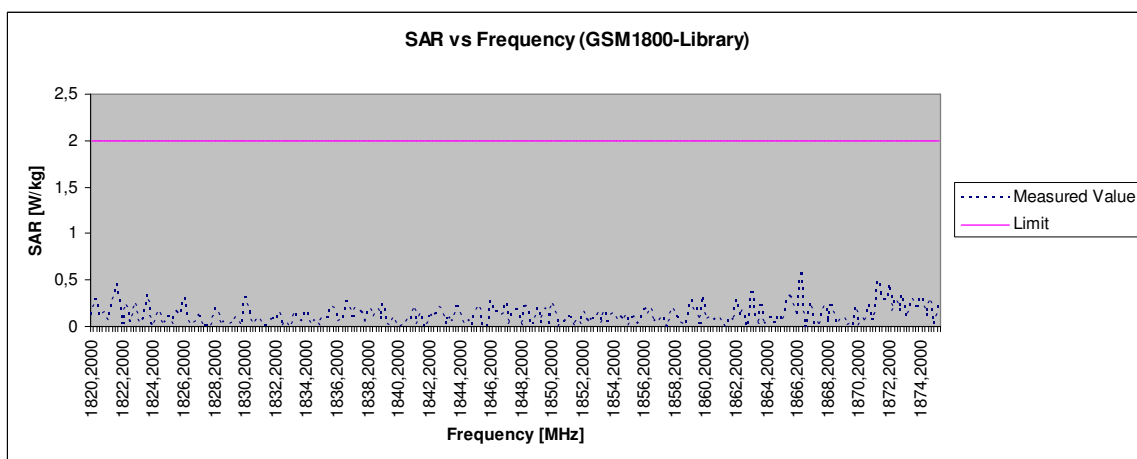
Fig. 4: Specific absorption rate measured at central library for GSM1800 signals
