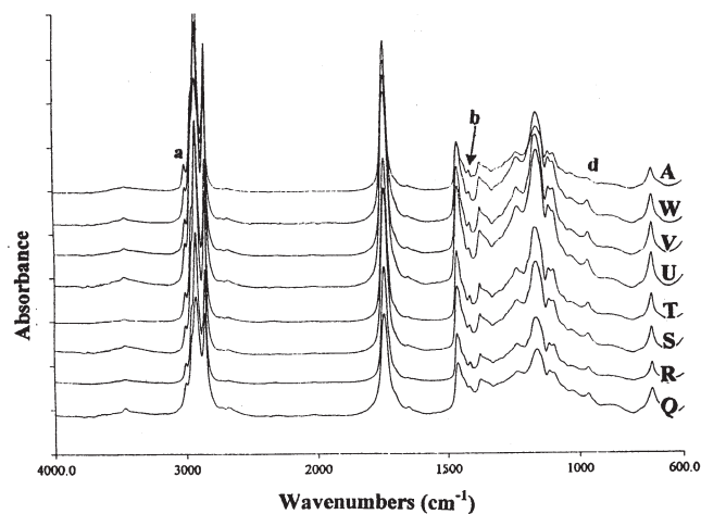
FIG. 20. FTIR spectra of (A) pure lard, (R)–(W) lard/CBF blends, and (Q) pure CBF. The percentages of lard in the blends are (R) 10, (S) 15, (T) 20, (U) 25, (V) 30, and (W) 35%. The labeled peaks (a, b, and d) are absorption bands that were used in the determination of lard in lard/CBF blends. See Figures 1 and 19 for abbreviations.
