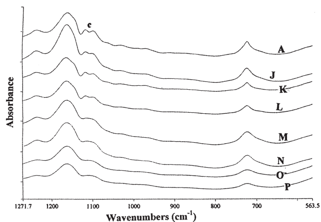
FIG. 17. FTIR spectra of (A) pure lard, (J)–(O) lard/CF blends, and (P) pure CF, illustrating changes in the absorbance values of the band in the region 1126\text{--}1085\text{ cm}^{-1} (c, Fig. 11). See Figures 1 and 11 for abbreviations; see Figure 12 for compositions of the blends.
