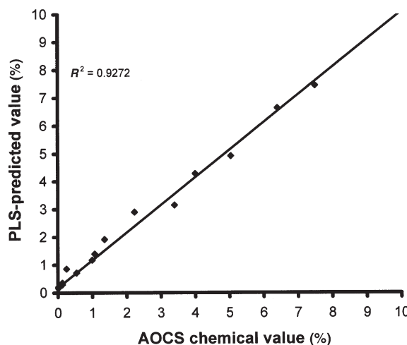
FIG. 4. Plot of actual vs. FTIR-predicted gossypol content in gossypol-spiked cottonseed oil for validation. For abbreviation see Figure 3.
