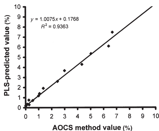
FIG. 3. Plot of gossypol content in gossypol-spiked cottonseed oil by AOCS chemical method (10) vs. partial least squares (PLS)-predicted values for calibration.
