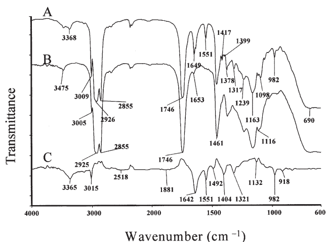
FIG. 1. IR spectra of (A) gossypol-spiked cottonseed oil, (B) pure cottonseed oil, and (C) the difference between A and B, representing gossypol only.
