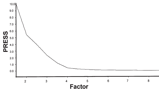
FIG. 5. Plot of predicted residual error sum of squares (PRESS) values vs. the different number of factors included in the cross-validation of the PLS model for gossypol content in gossypol-spiked cottonseed oil. For abbreviation see Figure 3.
