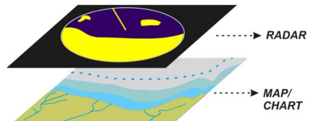
Figure 4. The overlay of radar image on the electronic chart. Since the chart contains only static data it can be handled as a common background image. In contrast to a dynamic background, such static image does not need any updates once it is uploaded into the video or graphic card's memory.
