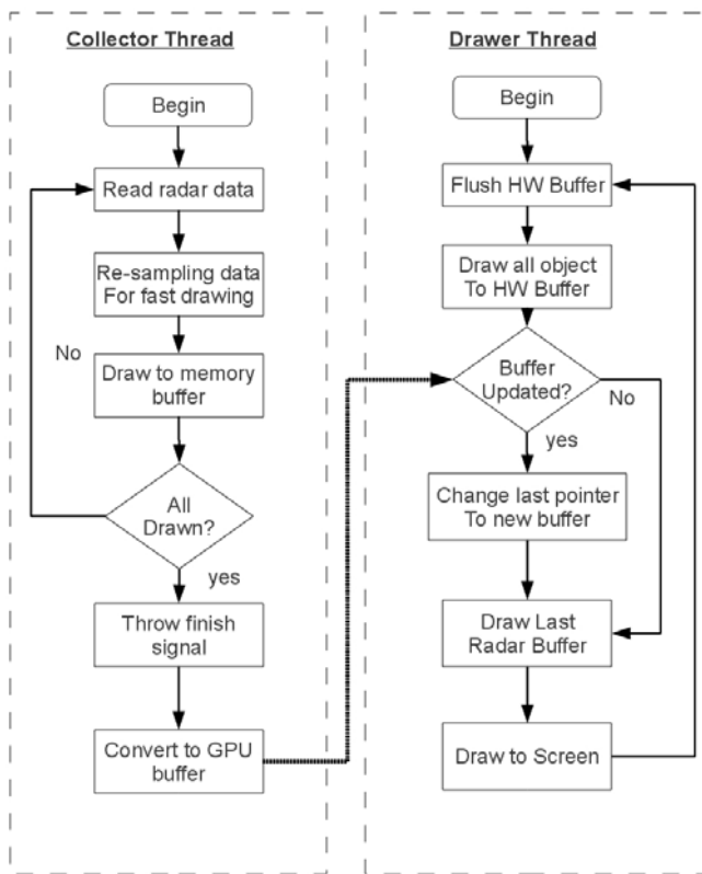
Figure 7. Multithreading strategy to handle large data streaming from radar. In order to overlay radar image on top of the electronic chart in real-time we have utilized two threads: collector and drawer thread. The first collector thread has a task to collecting, re-sampling and averaging data streaming from radar to be in line with the actual resolution of the display. The second drawer thread has a task to draw the final result of the overlay to the display screen.
