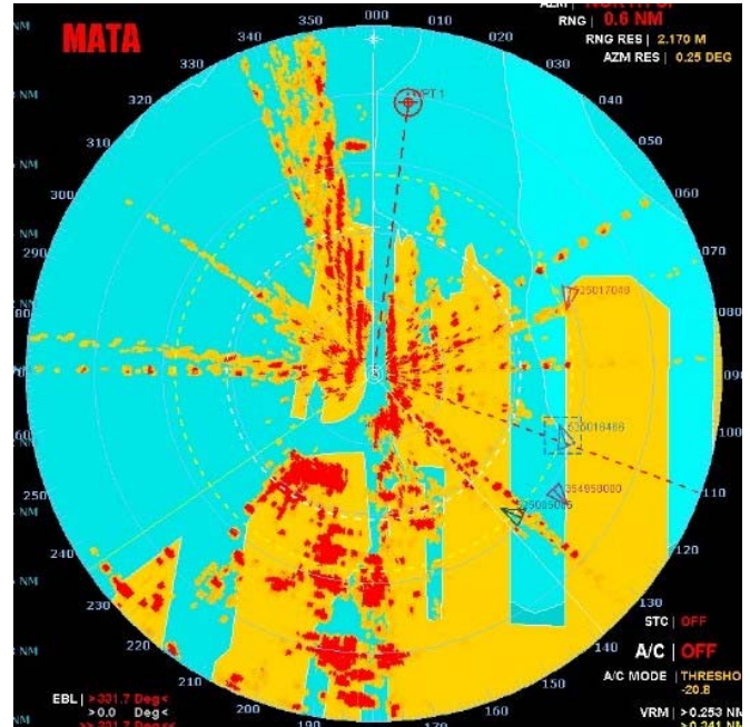
Figure 8. Result of the radar image overlay on the electronic chart. In this figure the overlay technique is applied directly on the PPI display of the radar INDERA MX-2. The overlaid radar (scattering) image is shown in red.
