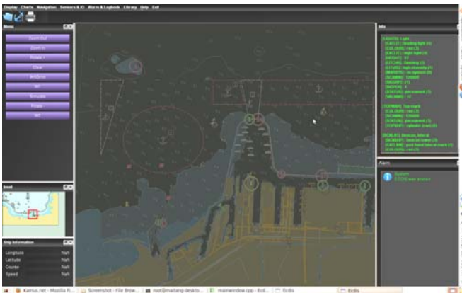
Figure 6. Display of ECDIS in the dusk color mode. The configurable chart display can be used to impressively enhance the effect of radar overlay technique.
