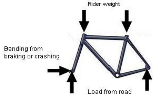
Figure 3 A free body stress diagram of a bicycle frame.
