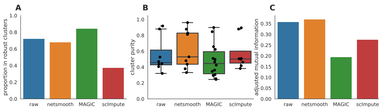
Figure 3. A) The proportion of cells which were assigned to robust clusters. B) cluster purity (proportion of dominant cell type) for the robust clusters. netSmooth produces the most pure clusters in terms of cell types. C) AMI of the clustering results obtained after application of each of the methods. Only netSmooth increases the AMI between the clustering and the cell types.
