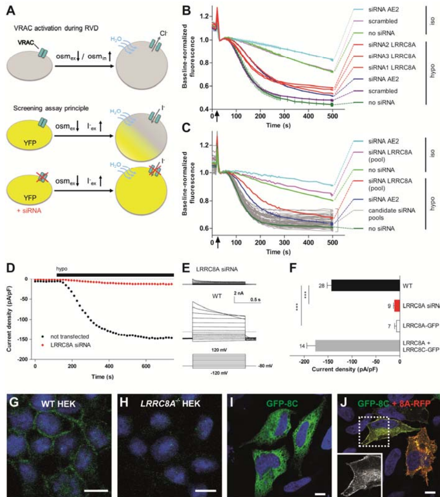
Fig. 1. siRNA screen for volume-regulated anion channel VRAC identifies LRRC8A. (A) Principle of screen. Top , in regulatory volume decrease (RVD) VRAC releases chloride. Below , quenching of YFP fluorescence by iodide entering through VRAC used as read-out. (B) Example traces, normalized to fluorescence at ~30-50 s. Averaged from wells treated with control siRNAs (scrambled, AE2, both n=3 ) and no siRNA ( n=2 ) (error bars, SEM), and individual traces from wells singly transfected with the 3 siRNAs against LRRC8A. Except for LRRC8A siRNA2 and 3, all traces are from the same plate. Arrow indicates addition of iodide-containing hypotonic (hypo; 229 mOsm) or isotonic (iso; 329 mOsm) saline. (C) Secondary screen using siRNA pools against candidate genes. Averaged control traces as above. (D) Typical time course of VRAC activation in WT or LRRC8A siRNA-treated HEK cells. Current densities at -80 mV are shown. Bar, application of hypotonic (240 mOsm) saline (hypo). (E) Current traces of fully activated I_{Cl(swell)} measured using the protocol shown below. Dotted lines indicate zero current. (F) I_{Cl(swell)} amplitudes (at -80 mV) of WT HEK cells, cells treated with LRRC8A siRNA, or transfected with indicated LRRC8 cDNAs. Error bars, SEM; number of experiments is indicated; ***, p<0.001 . (G) Plasma membrane localization of
