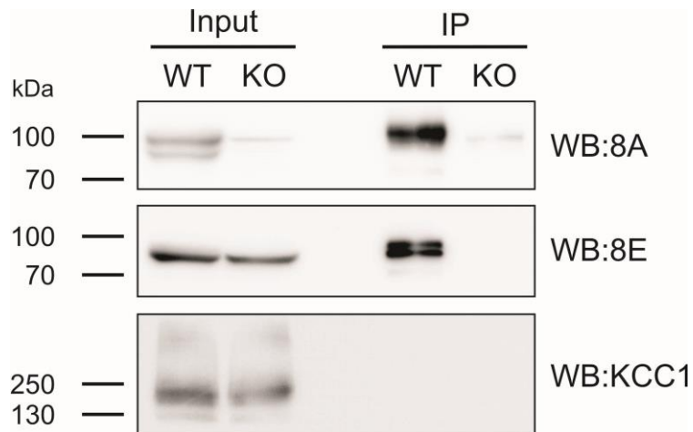
Fig. S8. Heteromerization of endogenous LRRRC8 proteins. LRRRC8A co-precipitated LRRRC8E (for which a suitable antibody was available) in immunoprecipitation with an LRRRC8A antibody from wild-type (WT) HEK cell lysate, but not from the LRRRC8A -/- knockout (KO, clone 3E7). The plasma membrane ion transporter KCC1 (negative control) did not co-precipitate with LRRRC8A. Lysate equivalent to 25% of input was loaded as reference (input).
