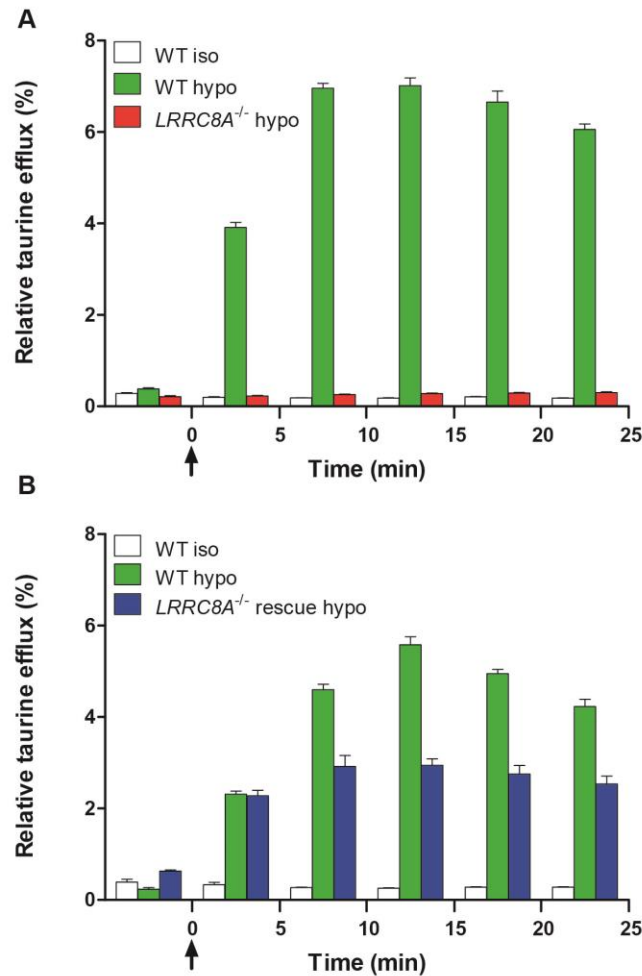
Fig. S9. LRRRC8A is crucial for swelling-induced 3 [H]-taurine efflux in HEK cells. (A) One set of wild-type (WT) HEK cells were in isotonic solution throughout, whereas another set of WT or LRRRC8A -/- HEK cells were exposed to hypotonic solution starting at t=0 (arrow). Bars represent means of 6 measurements of taurine efflux between the indicated time points. Error bars indicate SEM. (B) Taurine efflux measurement as in (A), but the LRRRC8A -/- HEK cells had been co-transfected with LRRRC8A and LRRRC8C-GFP. This co-transfection partially restores the taurine flux capability of LRRRC8A -/- HEK cells. Co-transfection was necessary as overexpression of LRRRC8A alone leads to a suppression of I_{Cl(swell)} . Only partial rescue of fluxes with transfected cells agrees with the transfection efficiency of roughly 50%.
