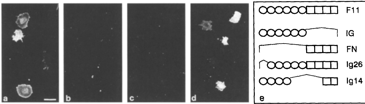
Figure 6. Binding of 2-3 FNIII-like domain of TN-R to F11 deletion polypeptides expressed on the surface of transfected COS cells. COS cells transfected with different F11 deletion constructs were grown to confluence. Monolayers comprising 5–25% transfected cells were incubated with bacterially expressed 2-3 FNIII domains of TN-R fused to glutathione-S-transferase. After washing and fixation, bound fusion protein was detected by immunofluorescence analysis using polyclonal antibodies directed to glutathione-S-transferase. (a) Construct IG comprising the Ig-related part of F11; (b) construct FN containing the FNIII-related domains of F11; (c) clone Ig26 lacking the aminoterminal domain of F11; (d) construct Ig14 lacking Ig-like domains 5 and 6 and the 1st and 2nd FNIII-related domains; (e) Schematic representation of mutant polypeptides of F11 used to narrow down the TN-R binding region on the F11 polypeptide. Ellipses symbolize Ig-like domains, and boxes represent FNIII-related repeats. \text{NH}_2 termini are on the left. Bar, 100 \mu\text{m} .
