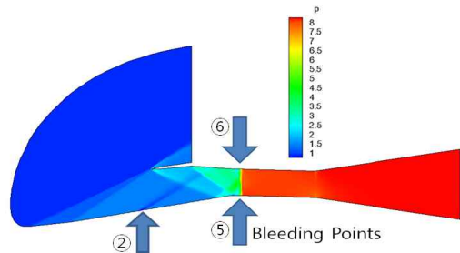
Fig. 12. Pressure distribution with bleeding at 3 places at M=2.5 , P_{back} = 12P_0
