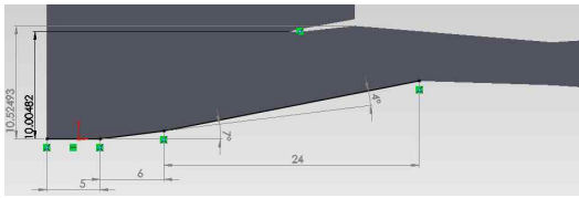
Fig. 2. Diagram of final model (length scale : cm, angle scale : degree)
