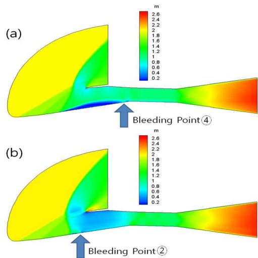
Fig. 8. Mach number distribution at M=2.0 ; (a) separation occurs even if bleeding is used (b) separation is removed
