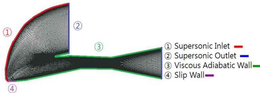
Fig. 3. One-block grid and boundary conditions
