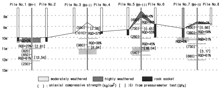
Fig. 5. Results of NX boring, pressurimeter test, and uniaxial compression tests.
