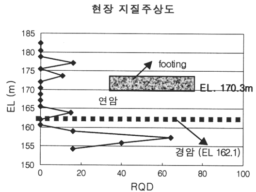
Fig. 20. RQD with depth and Elevation of Raft.
