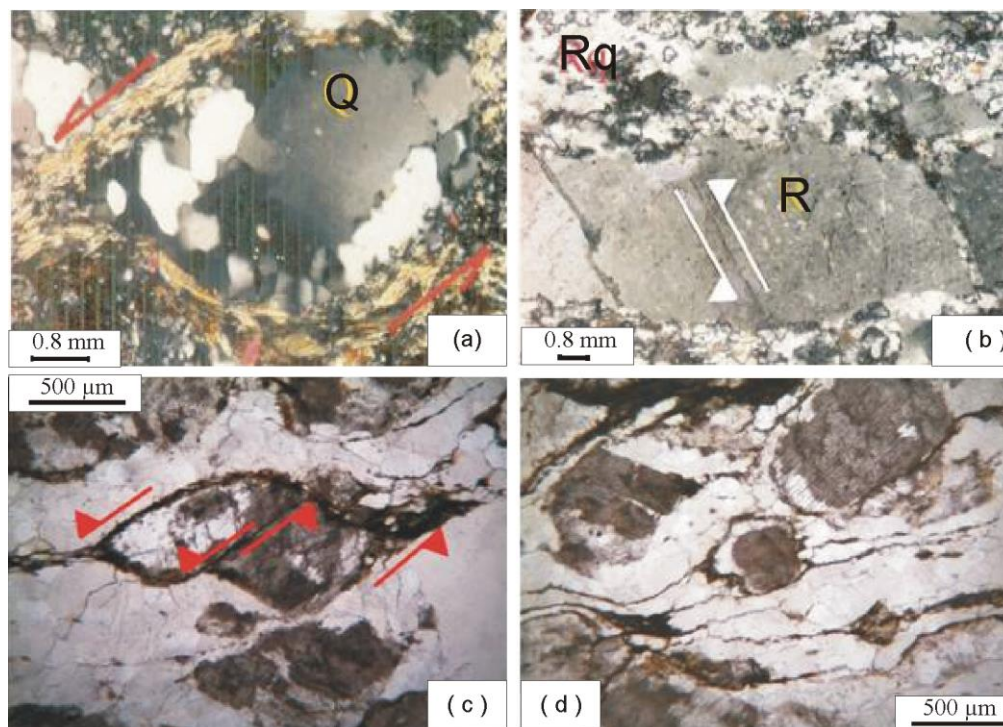
Figure 4: (a) \sigma_a mantled rotated porphyroclast of quartz (Q) forming pressure shadow and exhibiting sinistral sense of shear movement; (b) Ribbon of K–feldspar showing displaced microcracks (R) and dynamic recrystallisation quartz (Rq) in the marginal contacts; (c) \sigma_b mantled porphyroclast of K–feldspar displaced by microfaults and exhibiting bookshelf structures; (d) K–feldspar showing \delta type mantled porphyroclast and deciphering sinistral sense of shear movement.
