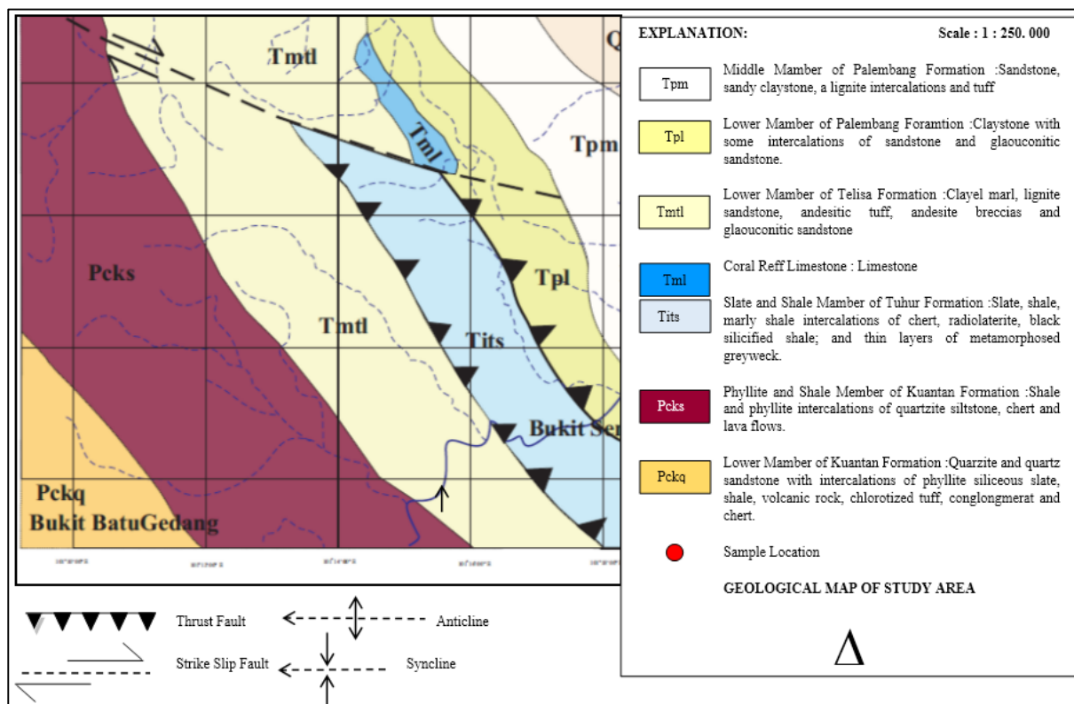
Fig 1. (above) Geological Maps of Rengat (Suwarna, Budhitrinsa, 1994); (below) Geological Maps of Solok (Silitonga, PH & Kastowo, 1994)
