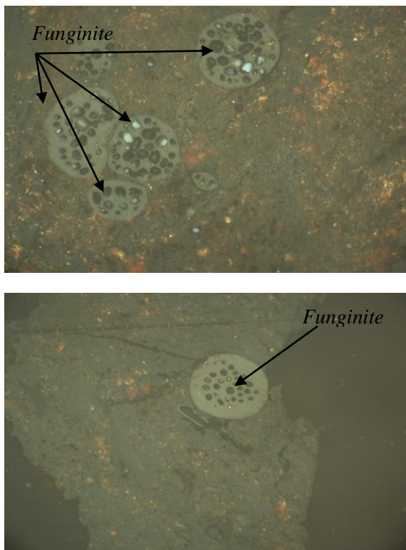
Fig. 3 (above) Funginite and mineral matter asosiasi with desmocollinite coal,reflectant white light, 500x. (below) Funginite asosiasi with desmocollinite coal, reflectant white light, 500x.
