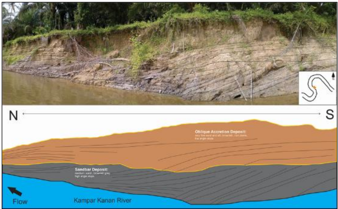
Fig 3. Deposit at western side of the river meander which shows sand bar deposit at bottom position with relative steep slope and deposit of oblique accretion at top with gentle slope than sand bar deposit.
