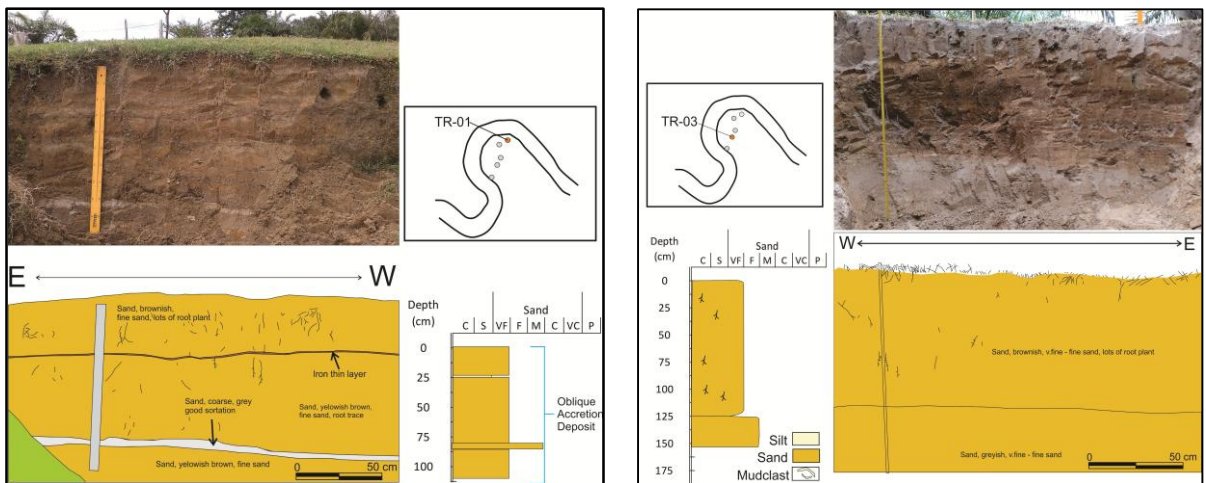
Fig 3. Deposit at western side of the river meander which shows sand bar deposit at bottom position with relative steep slope and deposit of oblique accretion at top with gentle slope than sand bar deposit.
