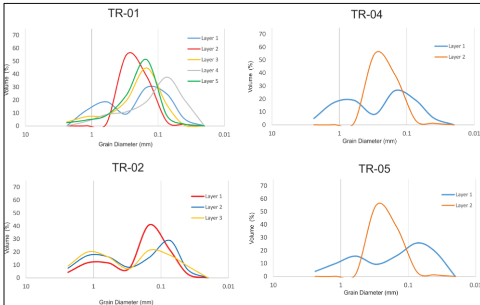
Fig 3. Sieve analysis that shows percentage of grain size distribution of each layer at four location (TR-01, TR-02, TR-04, and TR-05).
