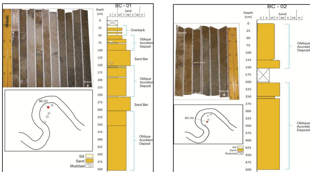
Fig 7. Analysis stratigraphy define from core data (BC-01 and BC-02) .
