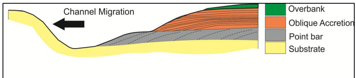
Fig 4. Model of stratigraphy in study area that related with Floodplain model with point bar (modified from Page, et al 2003).
