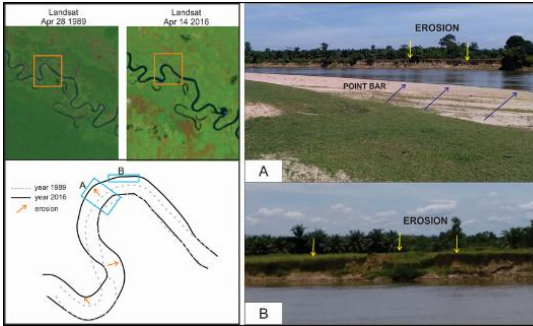
Fig 1. (A) Satellite image that showing geometrical changes the position of the river and image of point bar as result from river migration, and (B). Erosion at the northern side of the river.
