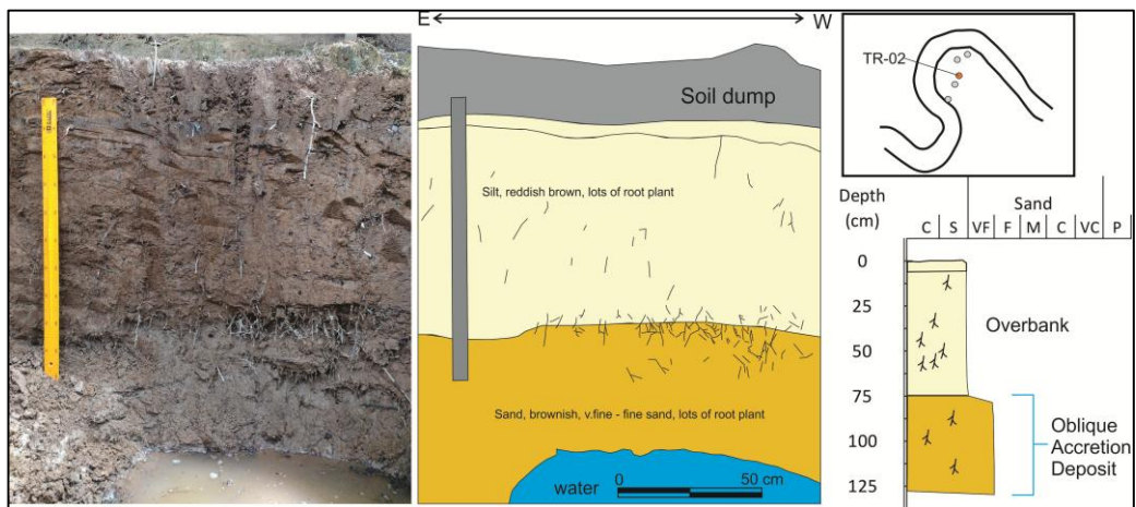
Fig 5. Succession at Trench (TR-02) that shows oblique accretion on bottom of the layer and overbank deposit at the top.
