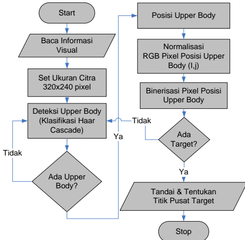
Gambar 5. Diagram alir pendeteksian target
