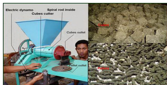
Figure 2. Cubing/Pelleting Equipment, Driven by Electric Dynamo Designed at the East Nusa Tenggara Assessment Institute for Agriculture Technology.
