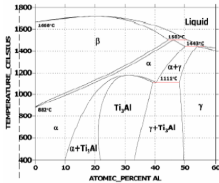
Fig. 1 The Ti-Al phase diagram [13]
