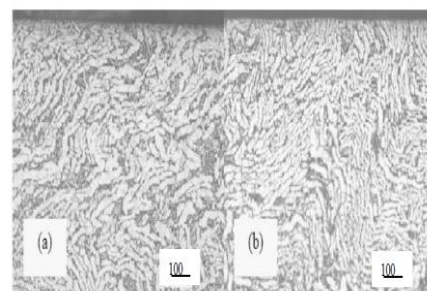
Fig. 3 Microstructure after machining at cutting speed of 55 m/min, feed rate of 0.15 mm/rev, depth of cut of 0.15 mm and CVD tool; (a) initial machining (b) end of machining.
