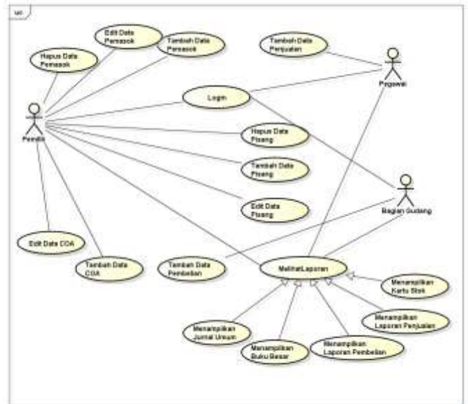
Gambar 1 Usecase Diagram
