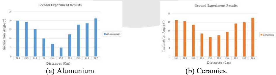
(a) Aluminium (b) Ceramics. Figure 3.6 The Second Experiment on inclination angle between 1 st sensor with 2 nd sensor
