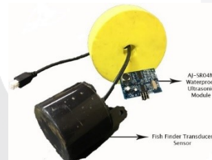
Figure 2.3 AJ-SR04M Waterproof Ultrasonic Module Combine with Fish Finder Transducer Sensor
