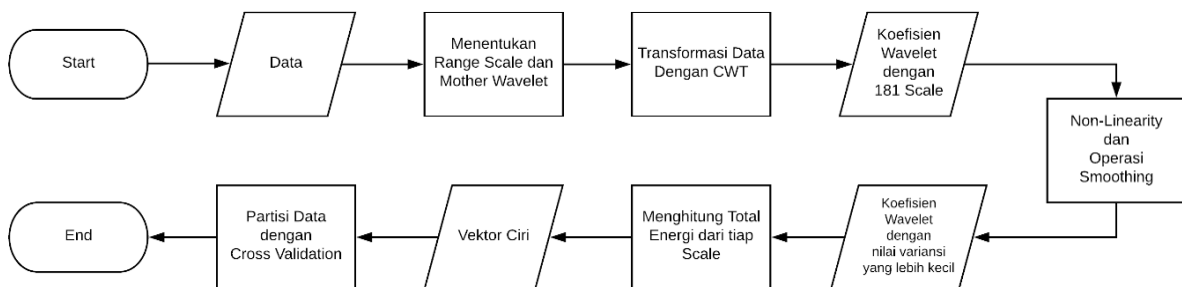
Gambar 3.3 Flowchart tahap preprocessing
