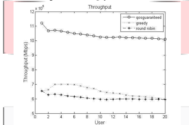
Gambar 8 Perbandingan nilai throughput MIMO 2x2 bandwidth 20 MHz
