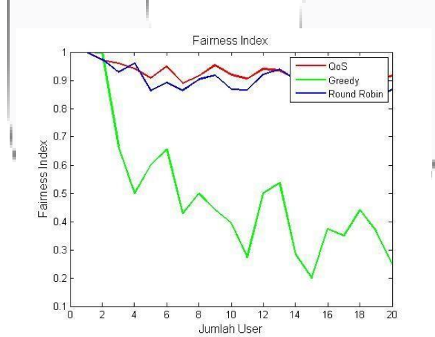
Gambar 9 Perbandingan nilai fairness MIMO 2x2 bandwidth 5 MHz
