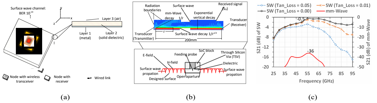
Figure 1: Proposed wireless communication fabric for WiNoCs. In Fig. 1(a) a dielectric-coated plane surface with a loss tangent \tan \delta is used. Fig. 1(b) shows transceiver and transducer (inverted quarter-wavelength monopole) components stacked over the CMOS-based 2-D waveguide sheet [2]. Fig. 1(c) represents the simulated S_{21} (dB) over wide-band frequency on the reactive surface with different lossy dielectric materials
