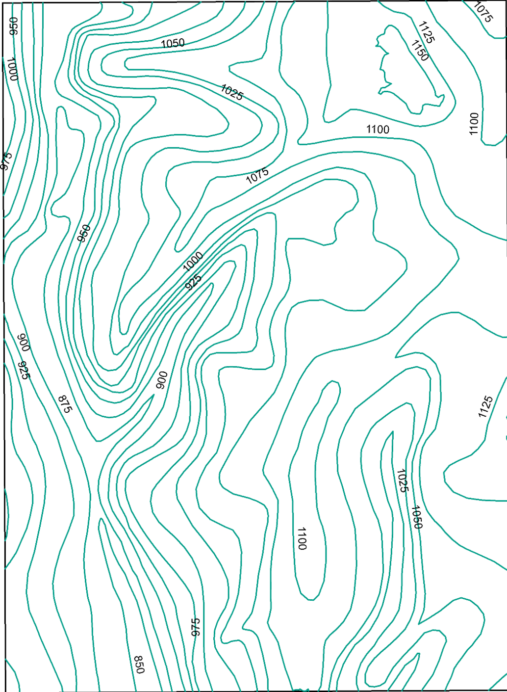
Fig. 3: The bedrock topographic map of the Colwell 7.5' Quadrangle with a 25' contour interval.
