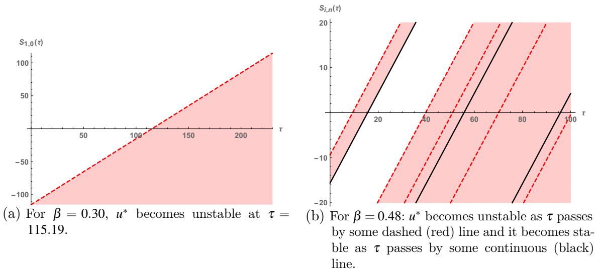
Figure 8 – The stability switch of u^* .
