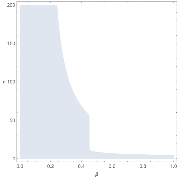
Figure 7 – Stability of u^* with respect to \beta and \tau .
