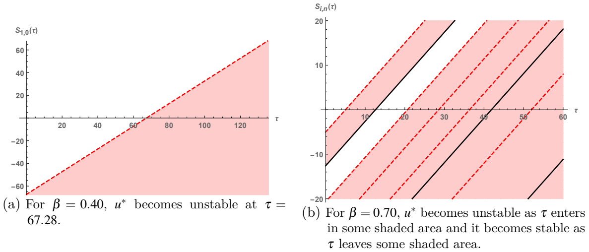
Figure 5 – The auxiliary function S_{i,n} and the stability switch of u^* .
