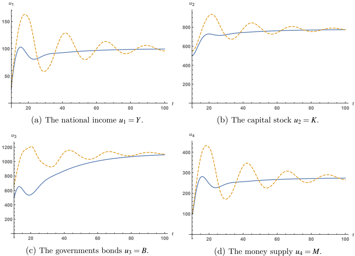
Figure 2 – The evolution in time with and without delay.
