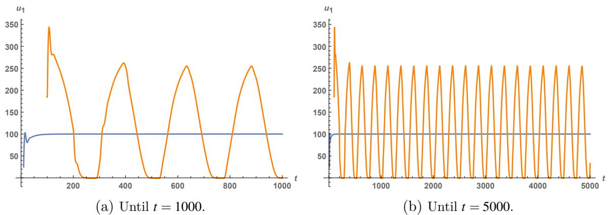
Figure 4 – The evolution of u_1 with \beta = 0.40 and \tau = 100 .
