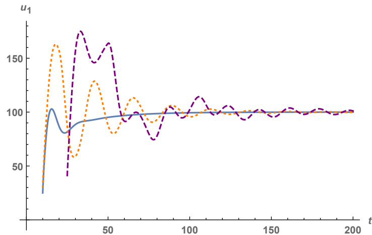
Figure 3 – The evolution of u_1(t) under different values of \tau .
