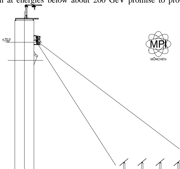
Figure 1: Setup of the experiment. A dedicated platform on the 70 m level of the central tower of the CESA-1 field houses four Winston cones which receive light from 13 - 18 heliostats in the field.
