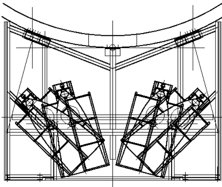
Figure 2: Location of light collecting cones with PMTs at the end (front diameter 1.06 m) in the platform seen from top. The tower is the curved structure on top.
