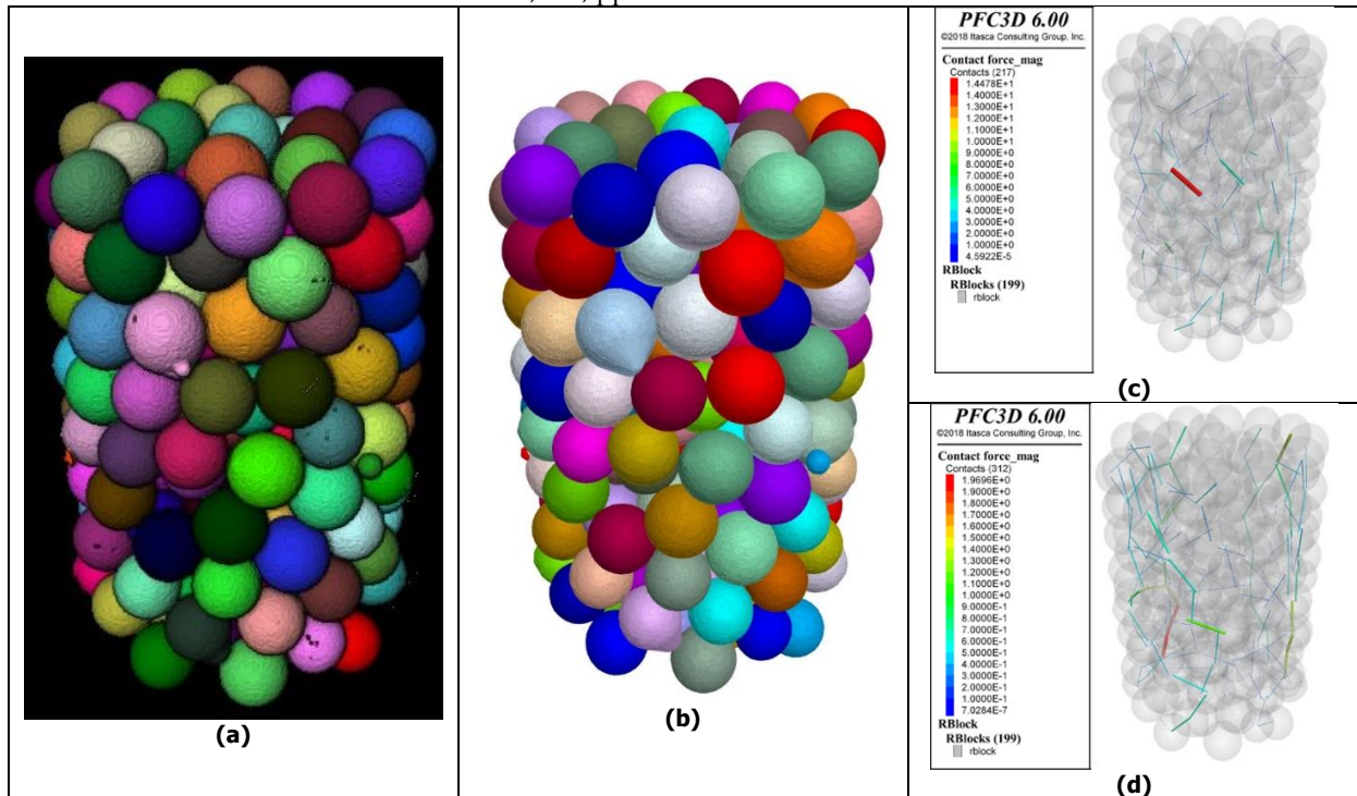
Figure 1: (a) Generated grain surfaces of the sample, (b) Generated particles in PFC from the grain surfaces, (c) Intergranular force after imposing particle displacements based on the measured particle velocities from the scan at uniaxial compressive stress of 5MPa to 10MPa, (d) Intergranular force after non-circumferential particle rearrangement due to the unbalanced forces
