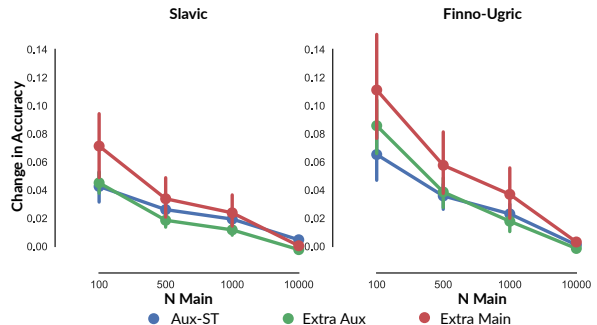
Figure 2: Results for UD treebanks.
