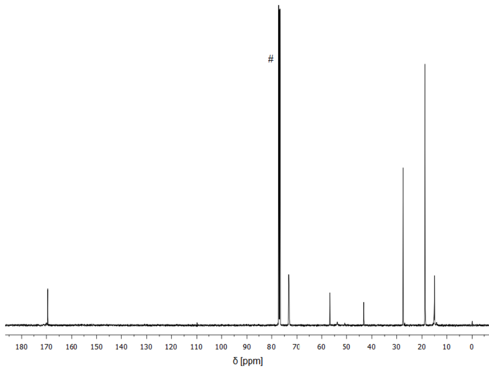
Fig. S10. ^{13}\text{C} NMR (500 MHz) spectrum of 3 in \text{CDCl}_3 ( \# solvent).
