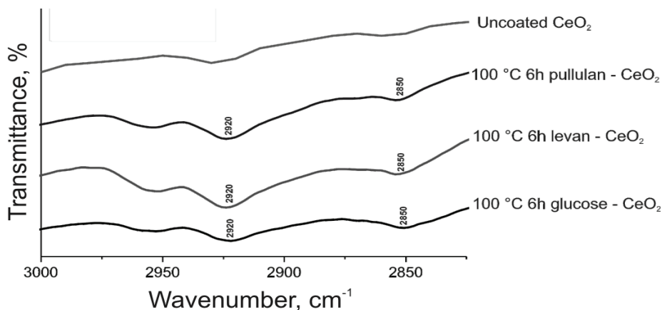
Fig. S-1. Enlarged FT-IR spectra region from 3000 to 2800 \text{cm}^{-1} of uncoated and CONPs coated with glucose, levan and pullulan by the SC method at 100 °C during 6 h.
