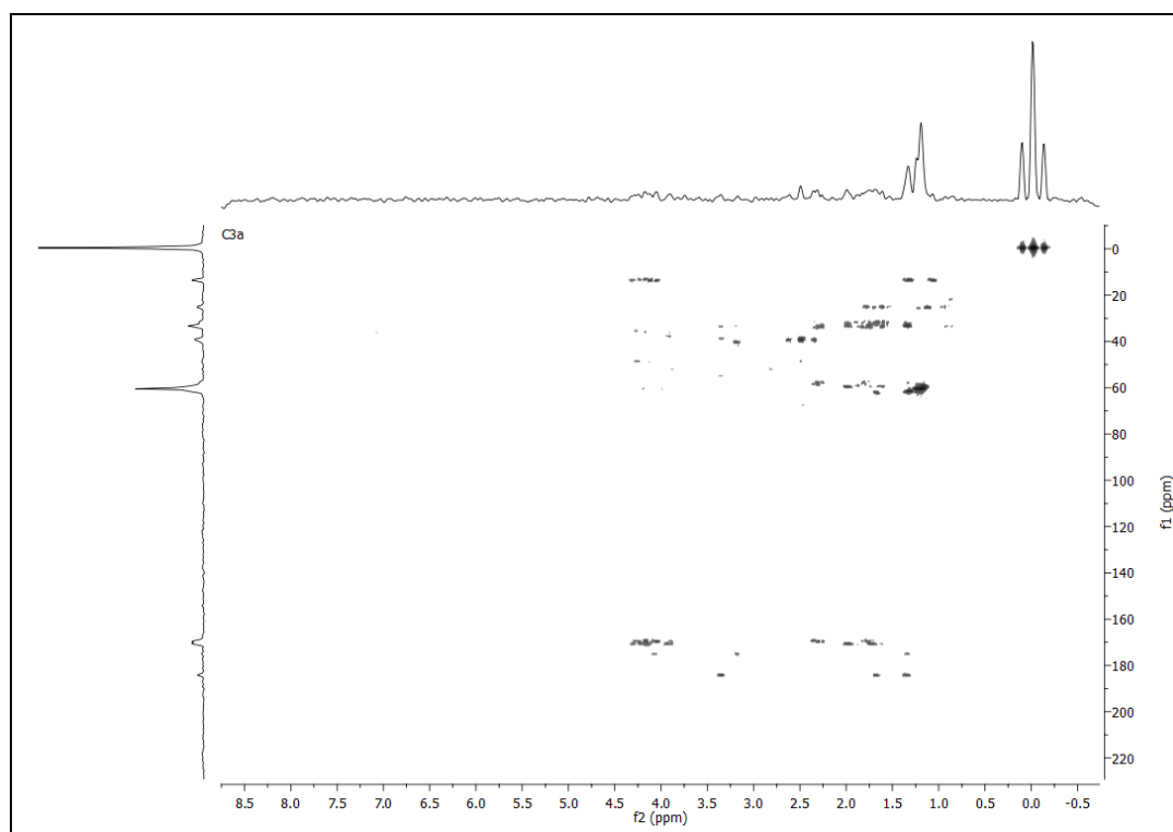
Fig. S14. HMBC spectrum of complex C3a
