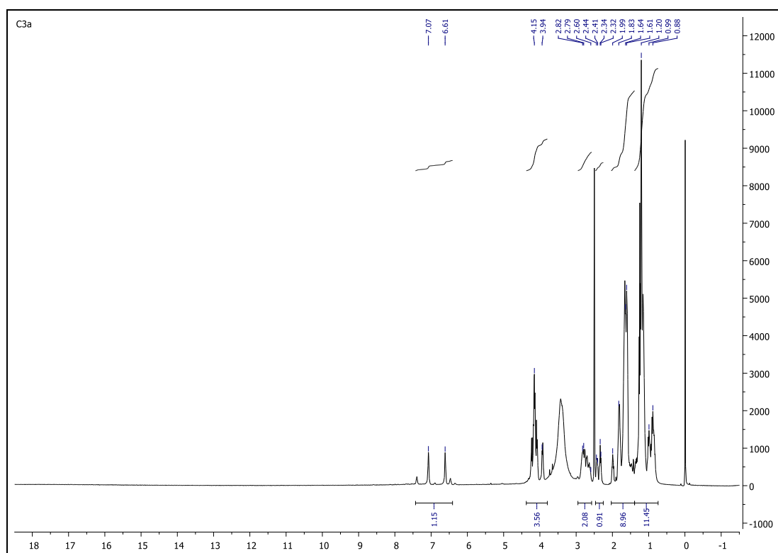
Fig. S12. ^1\text{H} NMR spectrum of complex C3a
