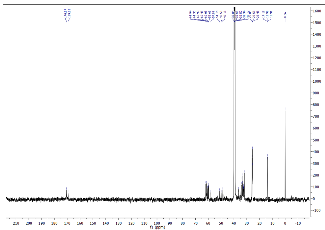
Fig. S16. ^{13}\text{C} NMR spectrum of complex C3b
