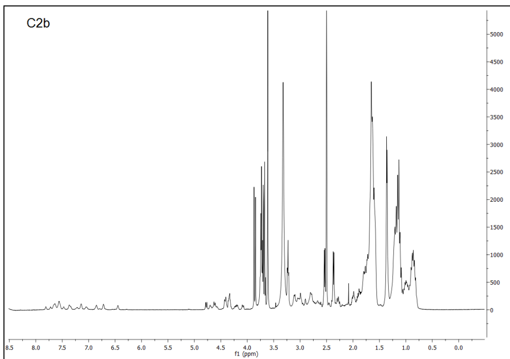
Fig. S9. 1 H NMR spectrum of complex C2b
