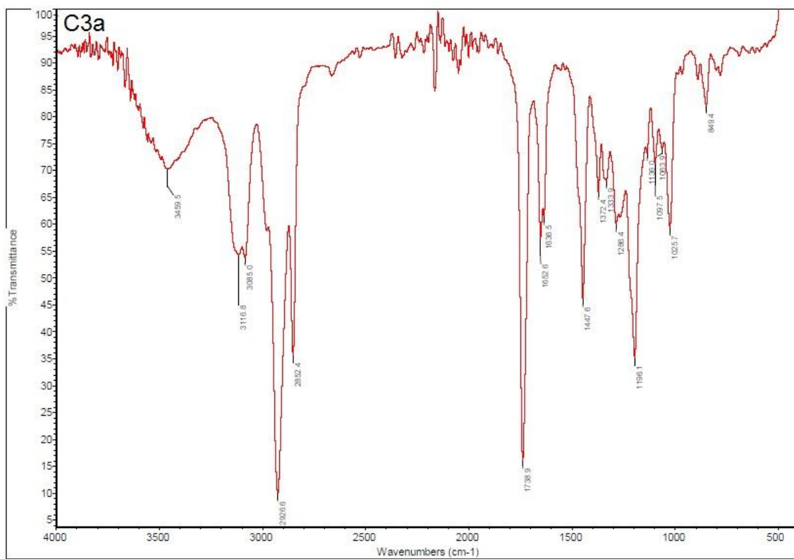
Fig. S2. FTIR spectrum of complex C3a
