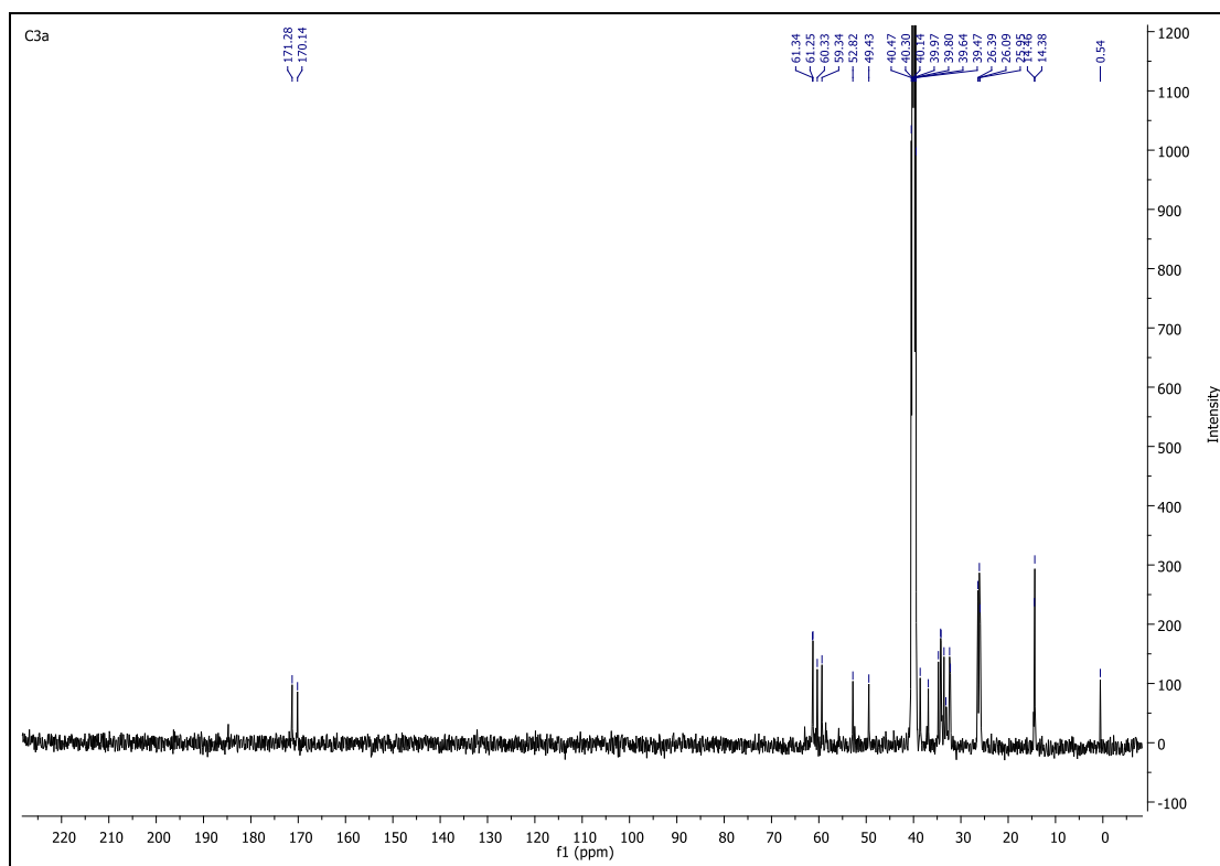
Fig. S13. ^{13}\text{C} NMR spectrum of complex C3a
