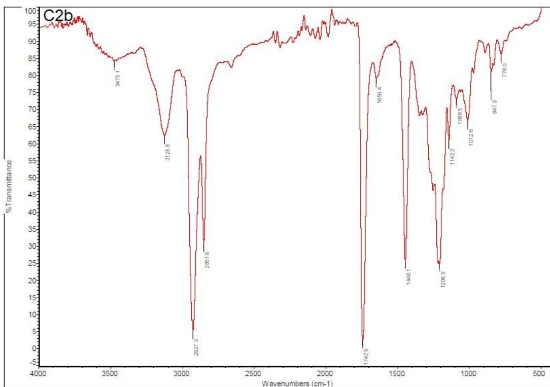
Fig. S3. FTIR spectrum of complex C2b
