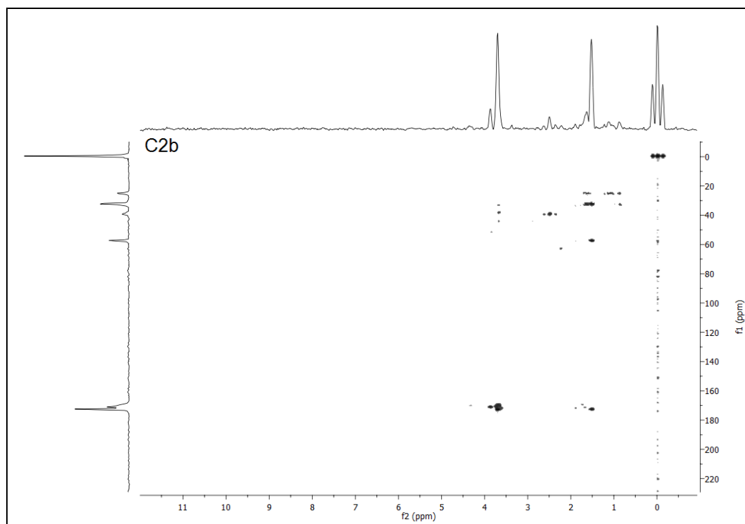
Fig. S11. HMBC spectrum of complex C2b
