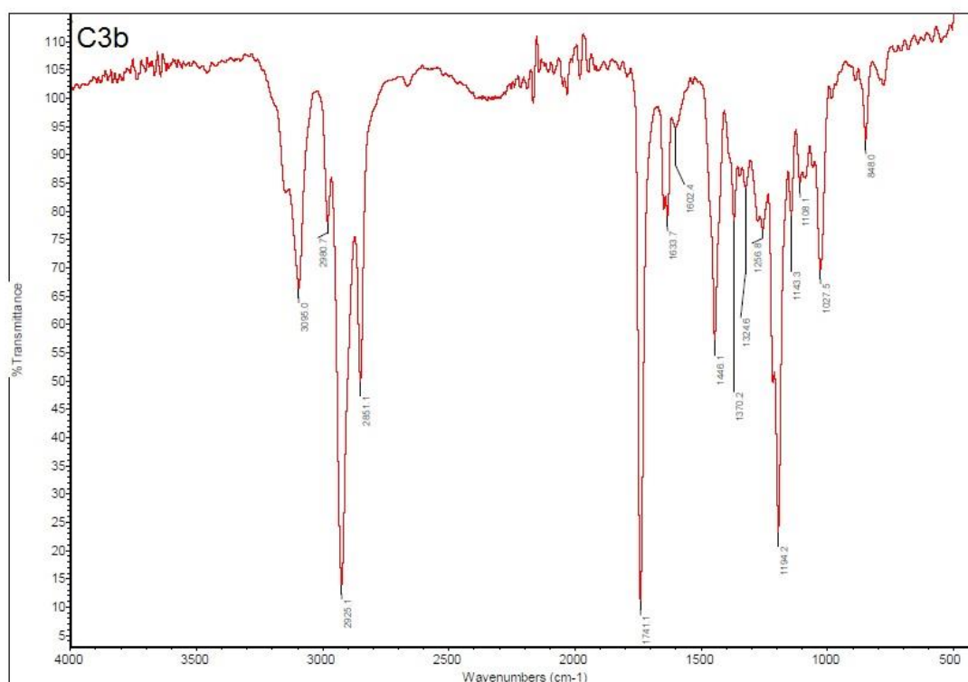
Fig. S4. FTIR spectrum of complex C3b
