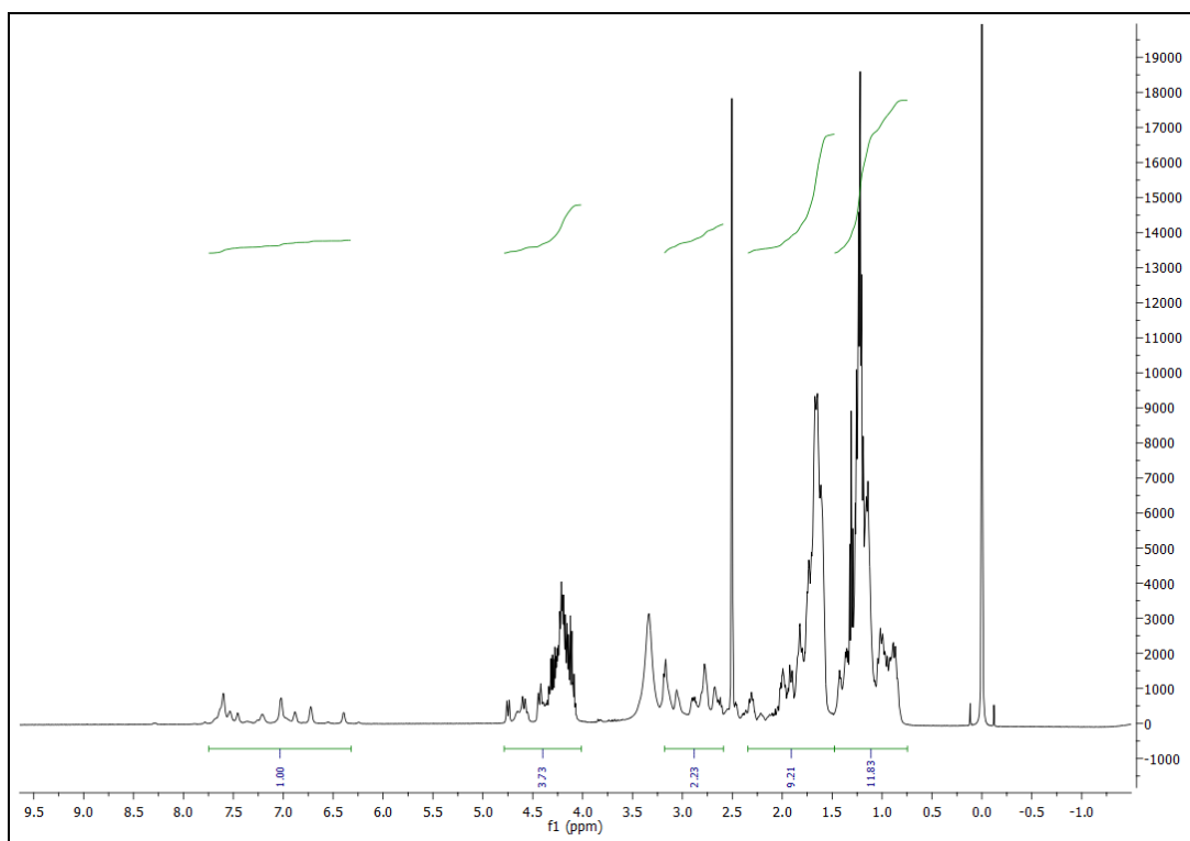
Fig. S15. ^1\text{H} NMR spectrum of complex C3b
