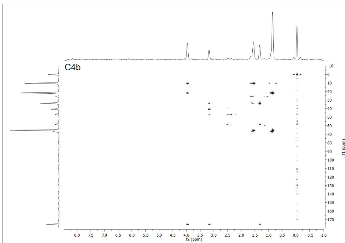
Fig. S20. HMBC spectrum of complex C4b
