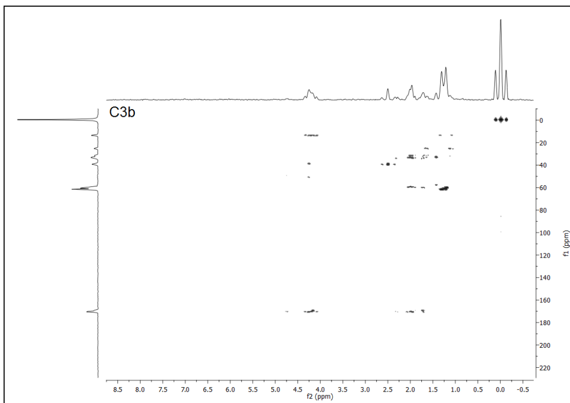
Fig. S17. HMBC spectrum of complex C3b
