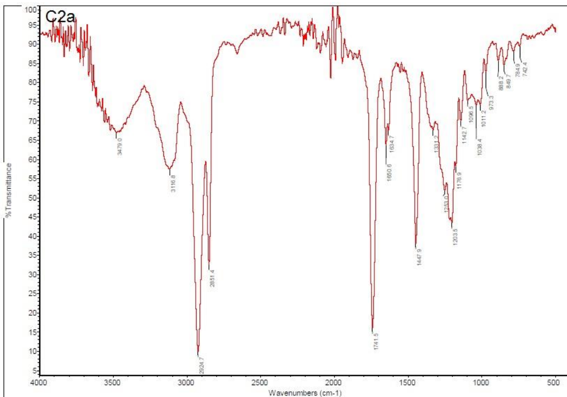
Fig. S1. FTIR spectrum of complex C2a
