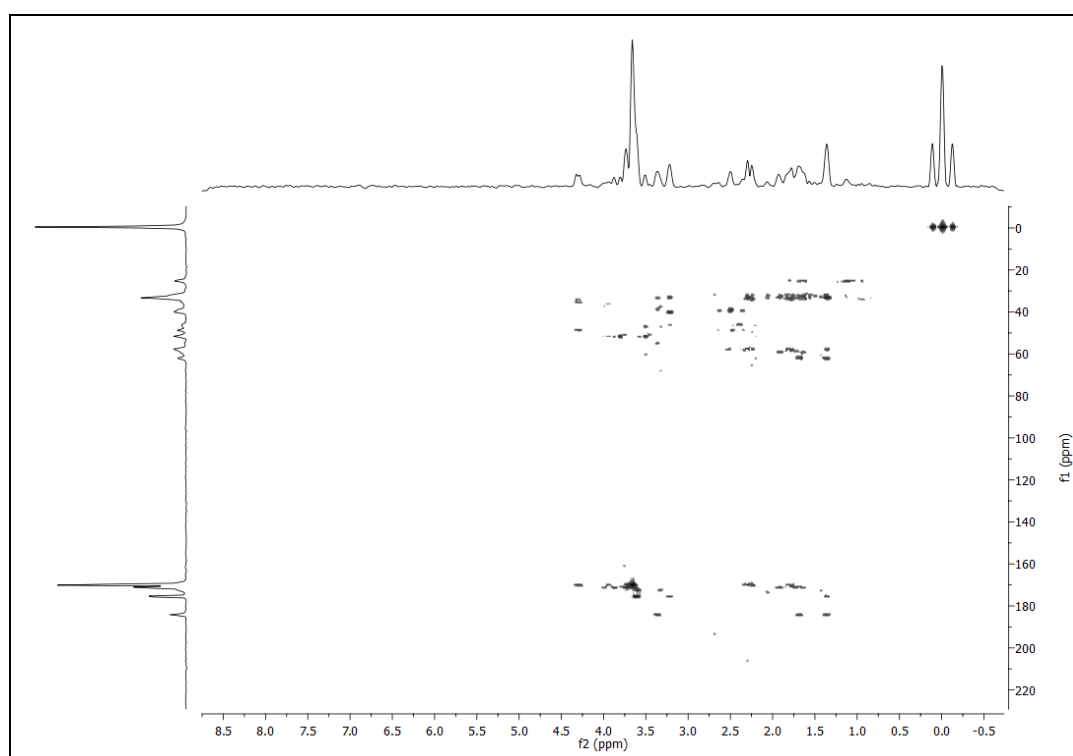
Fig. S8. HMBC spectrum of complex C2a
