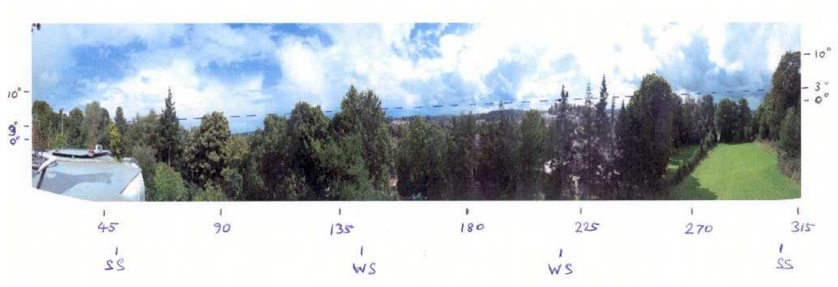
Plate 9b. A composite photograph of the horizon from northeast to northwest from the new (AD2000) sunshine tower, showing an approximate 3 degree altitude line and approximate azimuth limits of the Sun at the Winter and Summer Solstices when at 3 degrees altitude.
