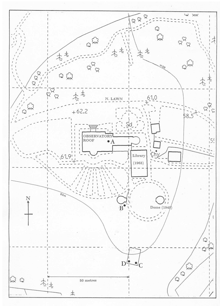
Figure 1. Map of the Grounds of Armagh Observatory showing the location of the sunshine recorder since 1880.
