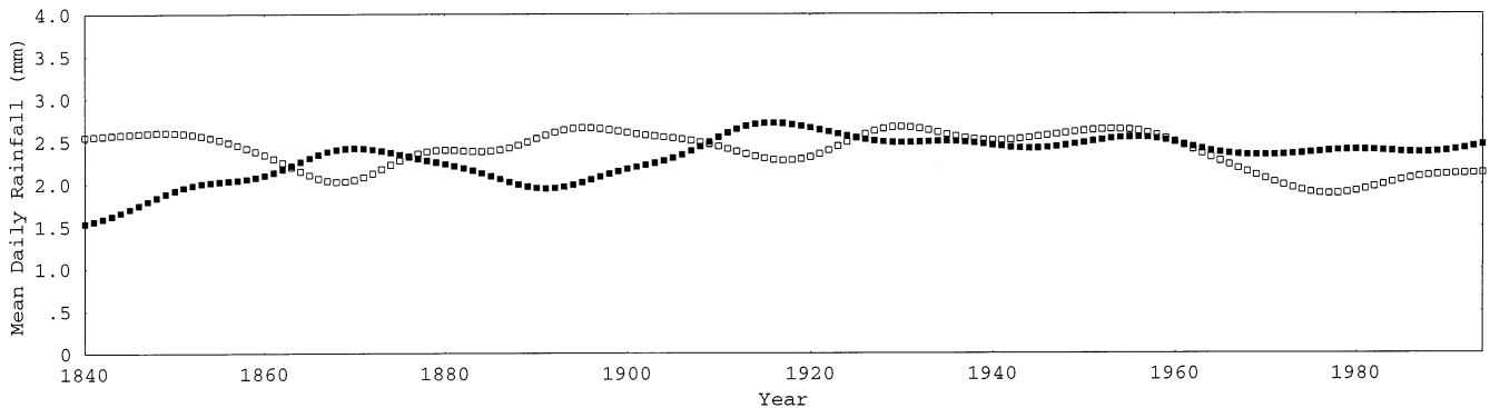
Fig. 5—Smoothed summer and winter precipitation against year (winter = solid squares; summer = open squares).
