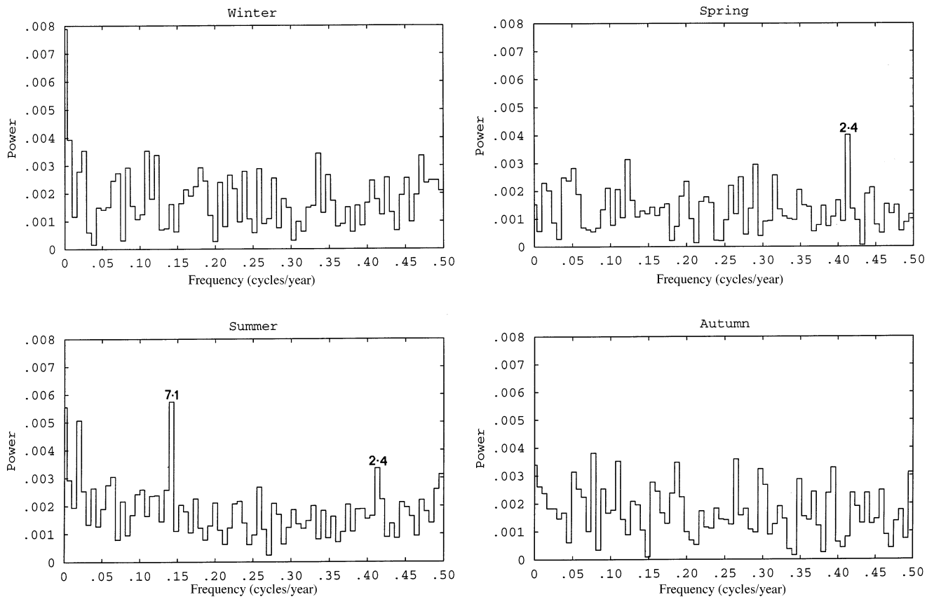
Fig. 6—Power spectra of mean seasonal precipitation. Note the periodicities of 2.4 years in the spring and summer series and 7.045 years in the summer series.
