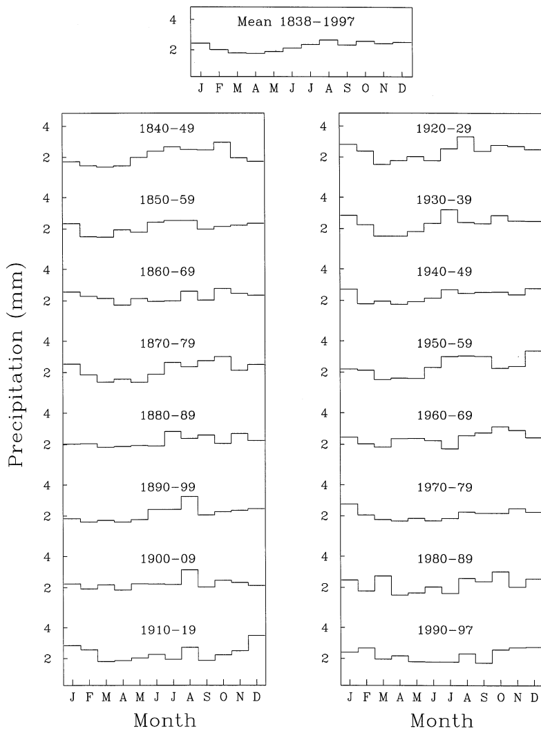
Fig. 2—Upper panel: mean daily precipitation per month for the period 1838–1997; lower panel: mean daily precipitation per month for decadal intervals, 1840–1997.
