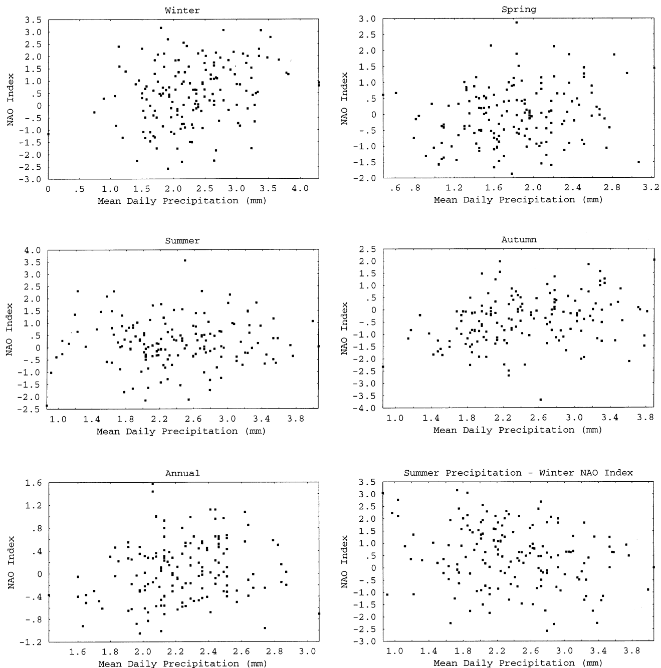
Fig. 7—Upper four panels: correlation of mean daily precipitation with the North Atlantic Oscillation index for each season; bottom left panel: correlation of annual mean daily precipitation with NAO index; bottom right panel: correlation of mean daily precipitation in summer with the NAO index for the previous winter.
