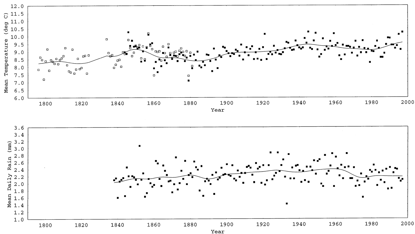
Fig. 3—Lower panel: solid squares = mean daily precipitation per year for the period 1838–1997; upper panel: mean temperature at Armagh, 1796–1996, from Butler and Johnston (1996) (open squares = Series I; solid squares = Series II). The smoothed curves are produced with a Gaussian smoothing function with a full width at half maximum of 11.8 years.
