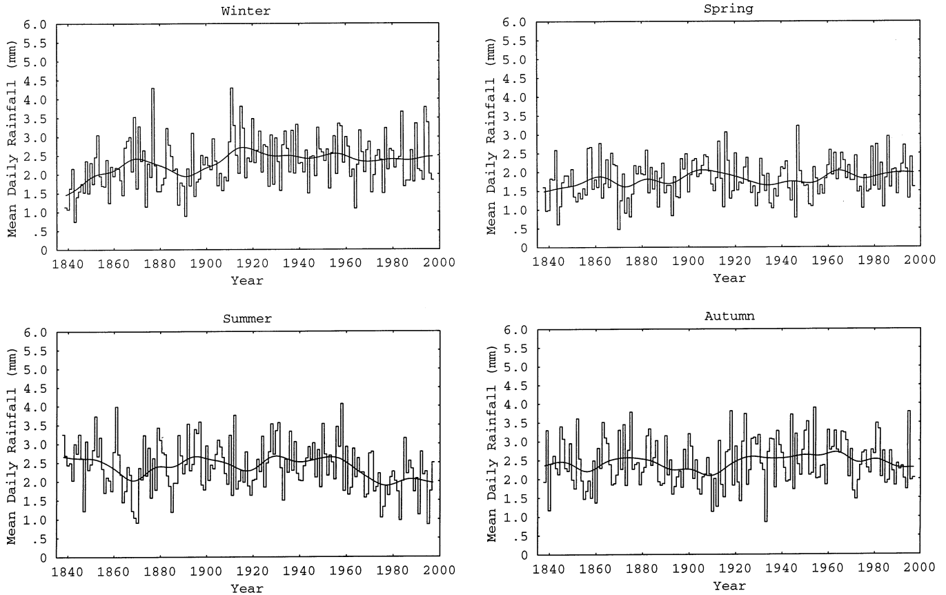
Fig. 4—Mean daily precipitation per season for the period 1838–1996 (smoothed curves as for Fig. 3).
