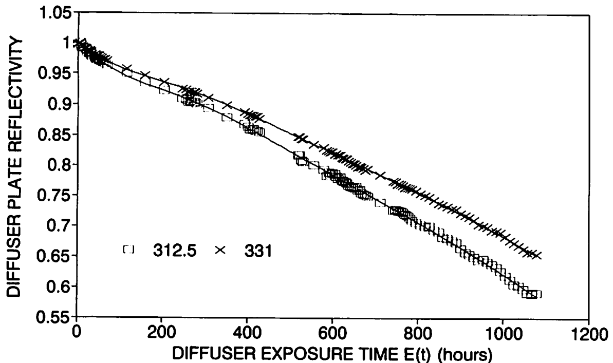
Figure 5.1. Total diffuser degradation as a function of accumulated solar exposure.
