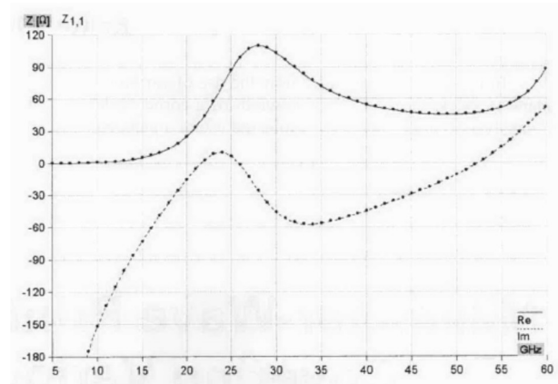
Figure 2: Real and imaginary parts of the pentagonal dipole impedance* as a function of frequency ( \epsilon_r=2.1 , h=0.254 mm, S^{**}=\lambda/4 ).
