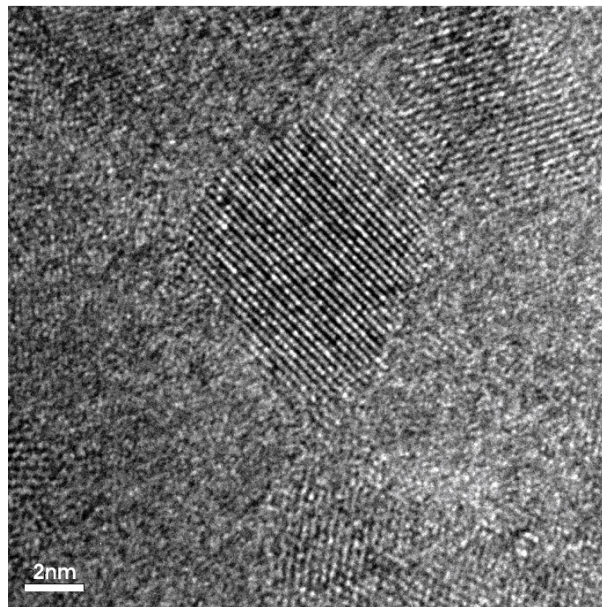
Fig.3 HREM nanograph of the investigated Nd-low Nd-Fe-B alloy in optimal magnetic state
