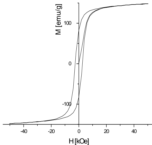
Fig. 4. Hysteresis loop of the investigated rapid quenched \text{Nd}_{4.5}\text{Fe}_{77}\text{B}_{18.5} alloy in the optimal magnetic state
