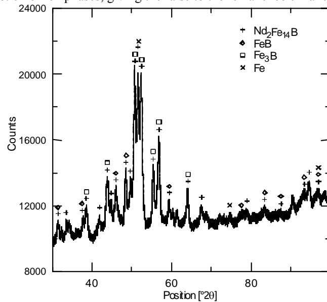
Fig. 1. X-Ray diffractogram of the investigated rapid quenched Nd_{4.5}Fe_{77}B_{18.5} alloy in the optimal magnetic state
