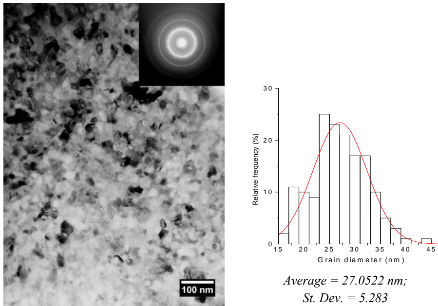
Fig 2. Bright field TEM micrograph of Nd_{4.5}Fe_{77}B_{18.5} alloy in optimal magnetic state with grain size distribution
