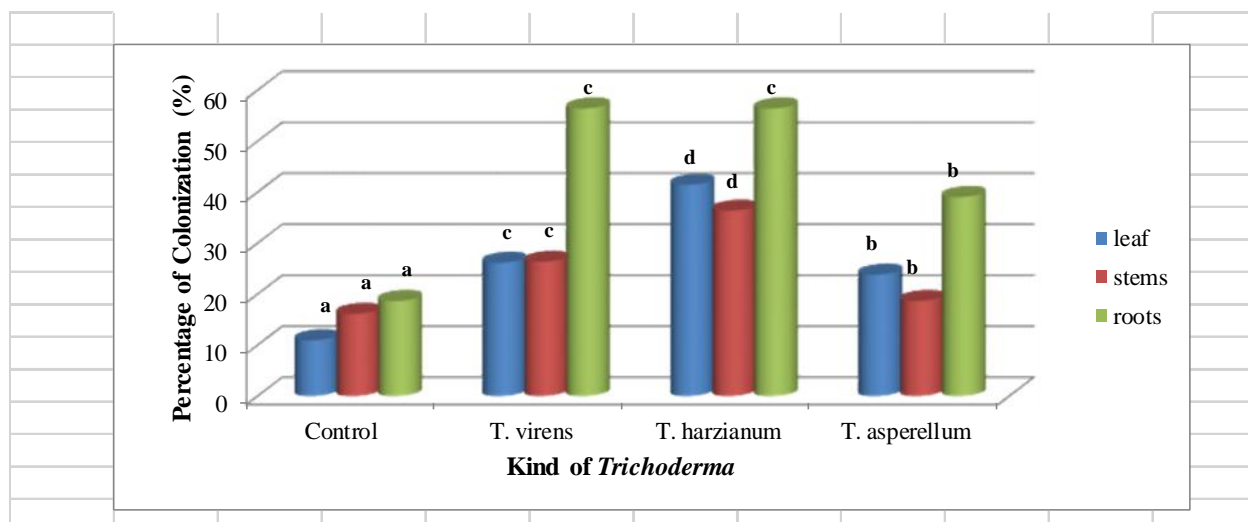
Figure 1. Percentage of Colonization Trichoderma on Cacao Seedlings Trichoderma species was not limited to the specific strains of Trichoderma shown. Trichoderma were isolated from colonized cacao seedlings after surface sterilization to verify that they were internally colonized. Low percentage Trichoderma was isolated from the un-inoculated control seedlings and pod compare with inoculated treatment. All three Trichoderma species studied were re-isolated from leaf, steam and root. Intermediate, with emerging Trichoderma hyphae then were observed and isolated. Trichoderma hyphae most often emerged from the surface outside (epidermis) but were also observed emerged from inside of pod. The percentage of isolating the inoculated Trichoderma strain from seedling with emerging hyphae was higher on T. harzianum and T. virens strains on this studied compare with T. asperellum and control. The Trichoderma isolated in highest percentage isolation of Trichoderma from each late samples were always consistent from root seedling
