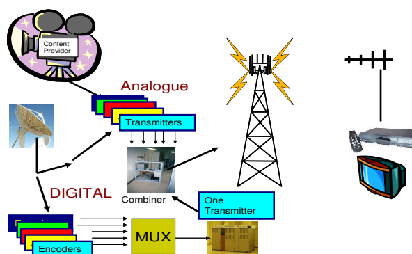
Figure 1 The scheme of DVB-T system (Roddy, 2006)
