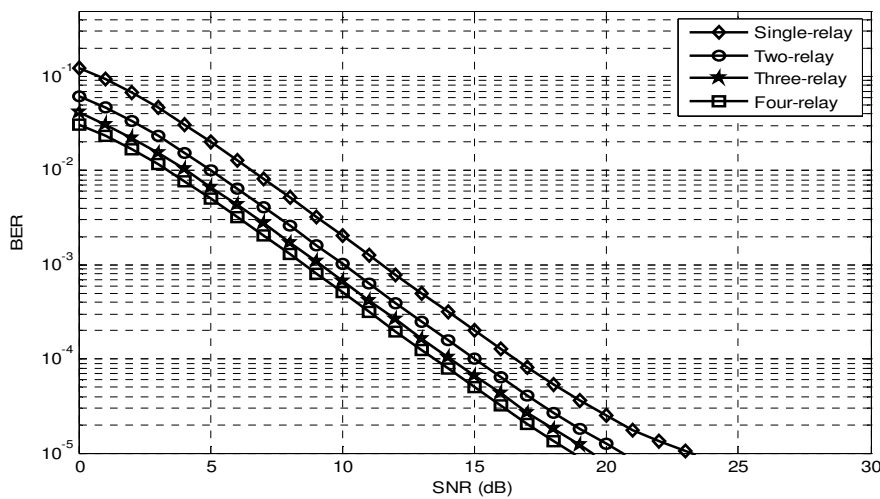
Figure 6. The BER performance for cooperative communication with convolutional encoder rate 1/3 and L = 3 .
