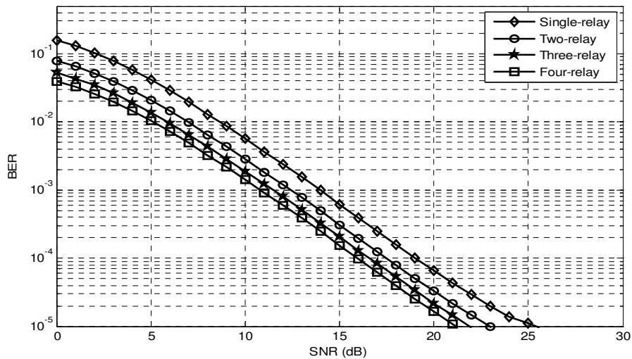
Figure 5. The BER performance for cooperative communication with convolutional encoder rate 1/2 and L = 3 .
