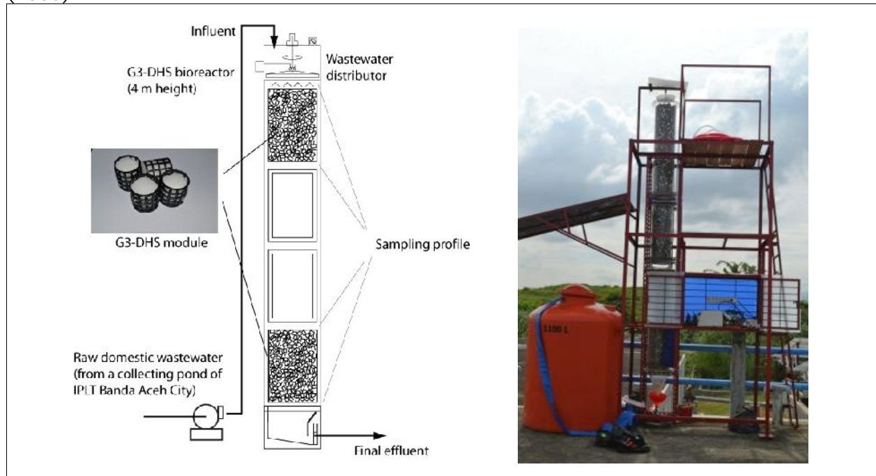
Figure 1. Schematic diagram and photograph of the G3-DHS bioreactor
