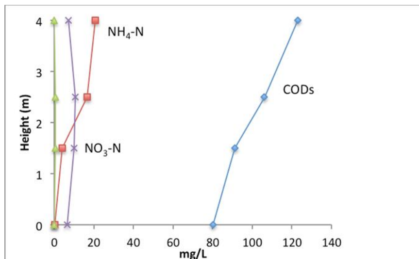
Figure 2. Profiles along the G3-DHS bioreactor height
