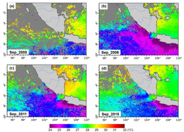
Figure 3-3: The distribution of SST (°C) in September during (a) 2005 (normal year), (b) 2006 (IOD+), (c) 2011 (IOD+), and (d) 2015 (IOD+).
