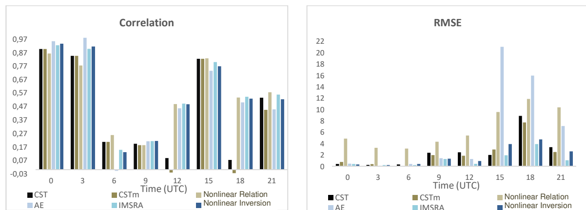
Figure 3-2: Graph of Correlation and RMSE between Estimated Rainfall and GSMaP in Muarateweh on Januari 2016
