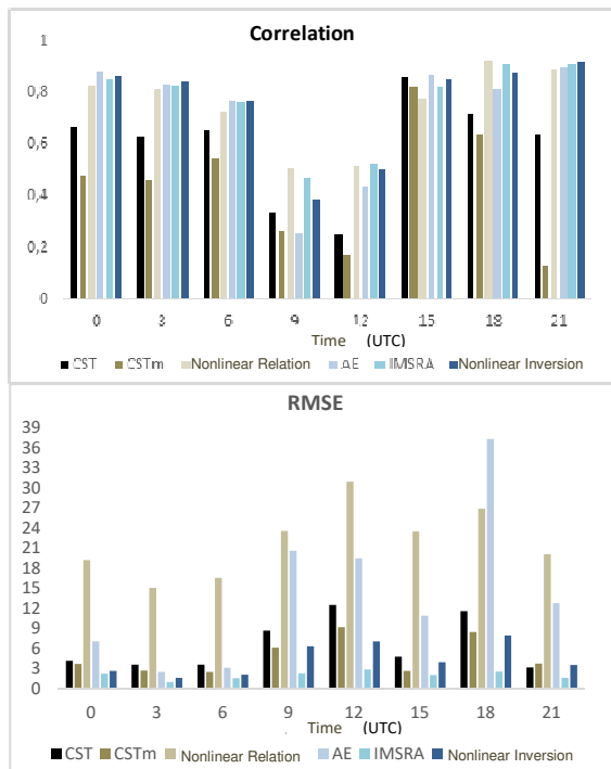
Figure 3-6: Graph of Correlation and RMSE between Estimated Rainfall and GSMaP in Palangka Raya in February 2016
