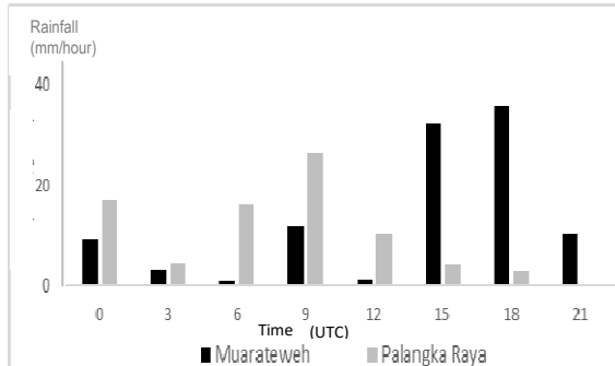
Figure 3-4: Timeseries of Total Rainfall from GSMaP Data in Muarateweh and Palangka Raya in January 2016
