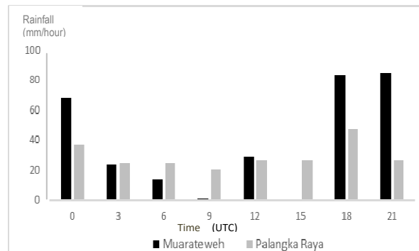
Figure 3-7: Timeseries of Total Rainfall from GSMaP Data in Muarateweh and Palangka Raya in February 2016
