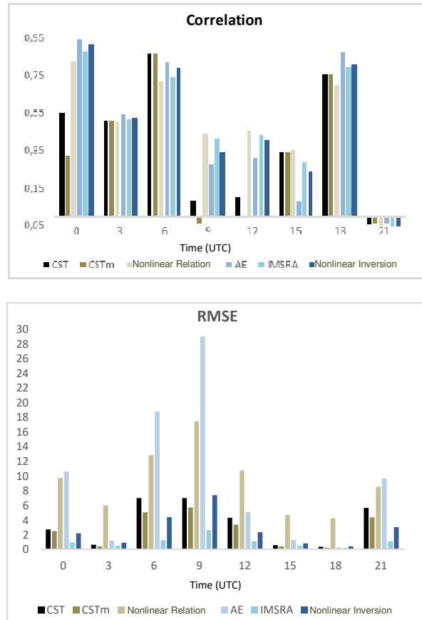
Figure 3-3: Graph of Correlation and RMSE between Estimated Rainfall and GSMaP in Palangka Raya on Januari 2016
