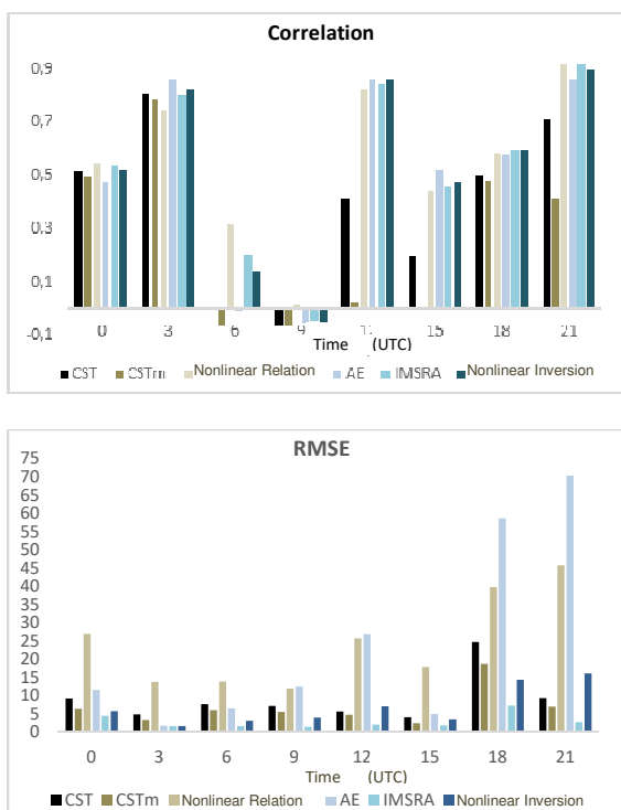
Figure 3-5: Graph of Correlation and RMSE between Estimated Rainfall and GSMaP on Muarateweh in February 2016
