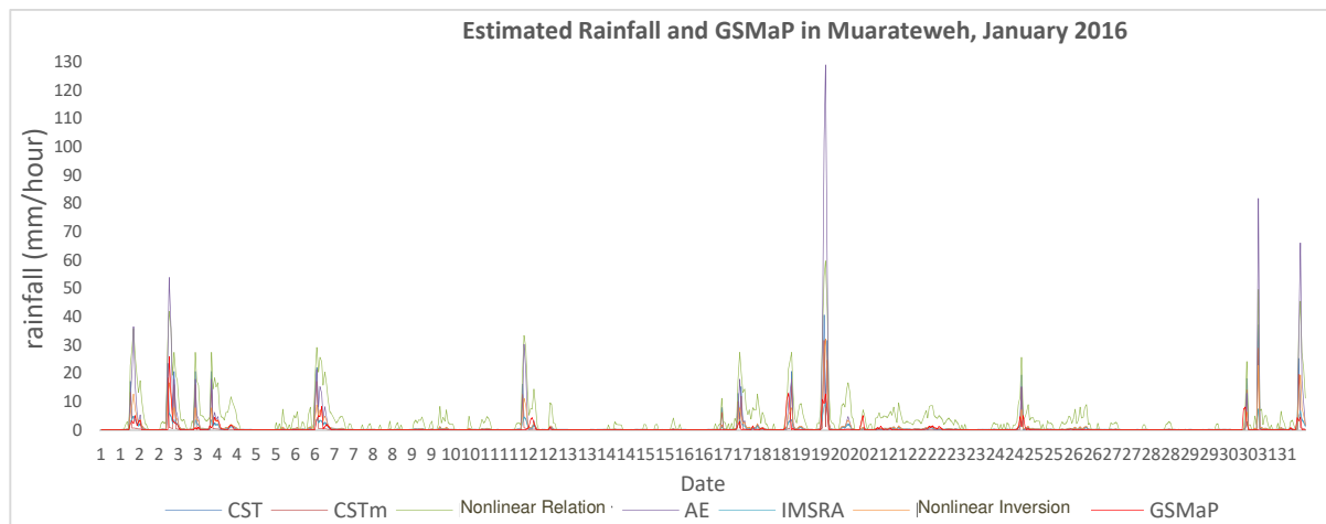
Figure 3-1: Graph of estimated rainfall and GSMaP in Muarateweh in January 2016
